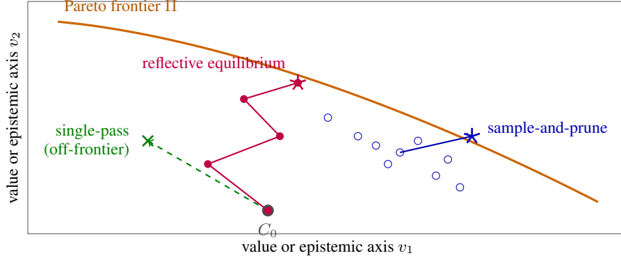
Figure 2: Reasoning as movement toward the Pareto frontier (schematic). The frontier II collects the defensible epistemic states. Different reasoning strategies trace different paths through the space. Reflective equilibrium walks dialectically from the initial commitments C_0 and ends at a frontier point. Sample-and-prune explores broadly and selects the non-dominated candidate. Single-pass abduction leaps once and may land in the dominated region. Shapes and trajectories are stylised, not derived from data.
