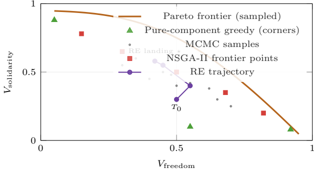
Figure 3: Ethical-value Pareto frontier. Projection of V(T) onto (V_{\text{freedom}}, V_{\text{solidarity}}) . Pure-component greedy baselines collapse to corners; NSGA-II traces the frontier; RE lands at an interior frontier point — a defensibly mixed normative profile.
