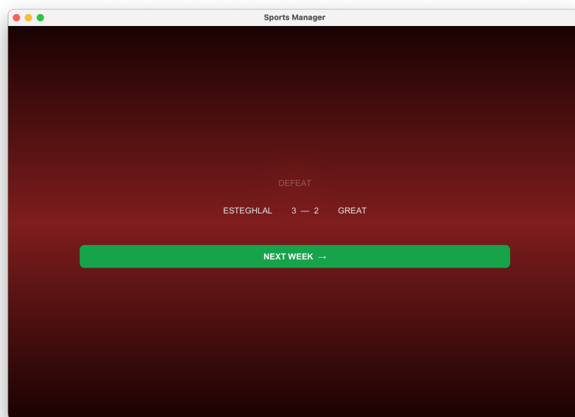
Figure 9: Post-Match Screen
