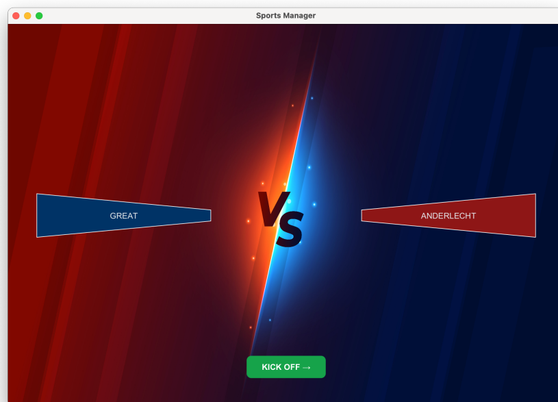
Figure 5: Versus Screen
