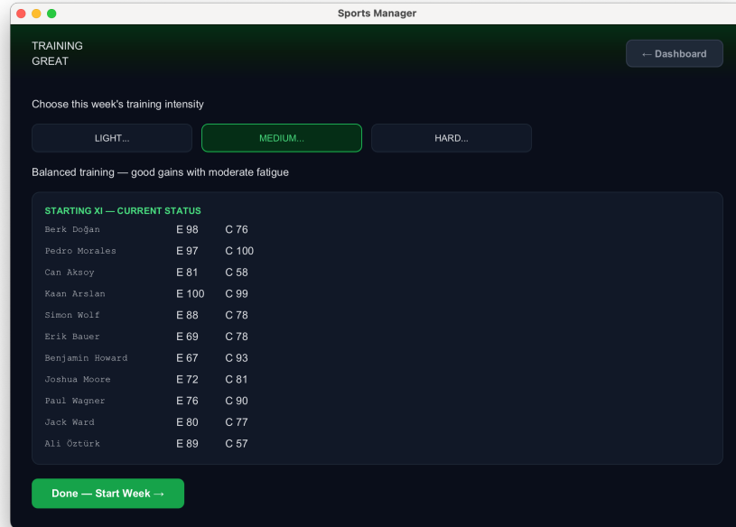
Figure 4: Training Screen
