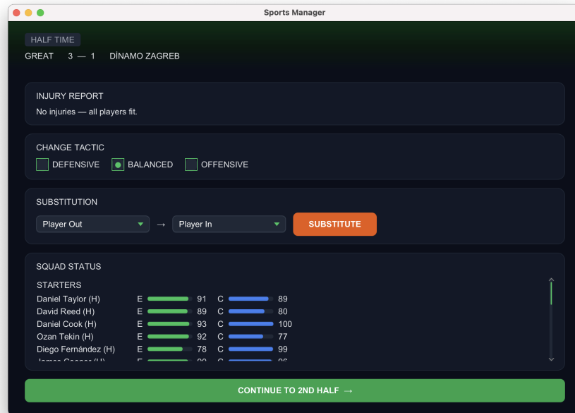
Figure 8: Half-Time Screen
