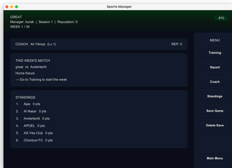
Figure 3: Dashboard Screen
