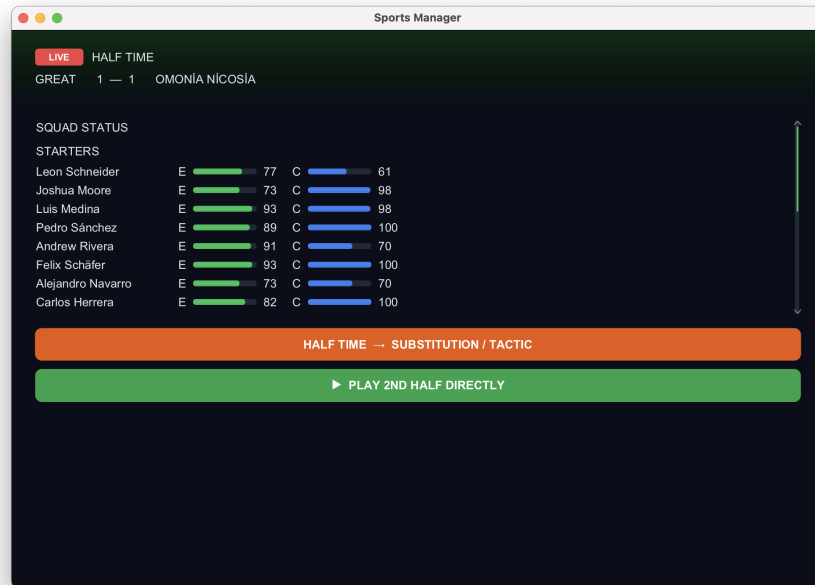
Figure 7: Match Screen
