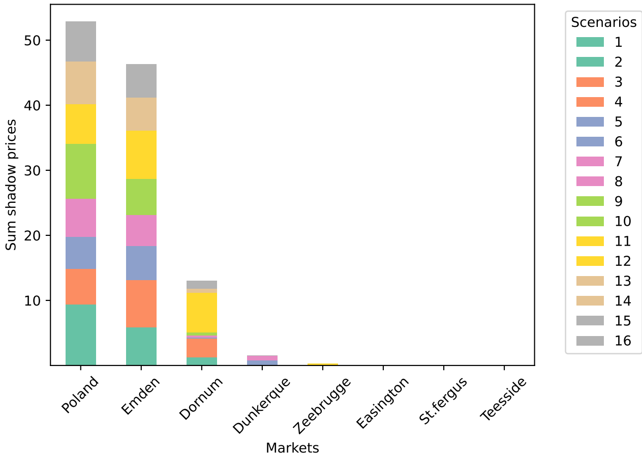
Sensitivity analysis
