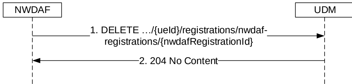
Figure 5.3.2.4.8-1: NWDAF deregistration
