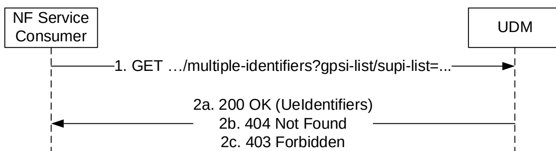
Figure 5.2.2.25: GPSIs/SUPIs Translation
