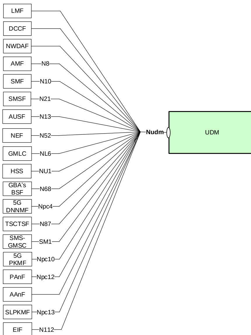
Figure 4.1-1: Reference model – UDM
