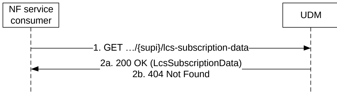
Figure 5.2.2.27-1: Requesting a UE's LCS Subscription Data
