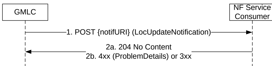
Figure 5.2.2.6.1-1: LocationUpdateNotify Notification
