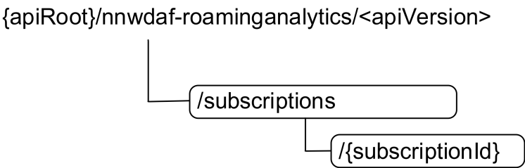
Figure 5.8.3.1-1: Resource URI structure of the Nnwdaf_RoamingAnalytics API
