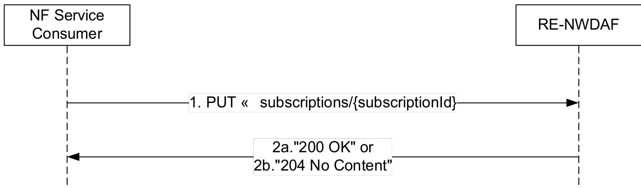
Figure 4.9.2.3-1: NF service consumer updates subscription to notifications
