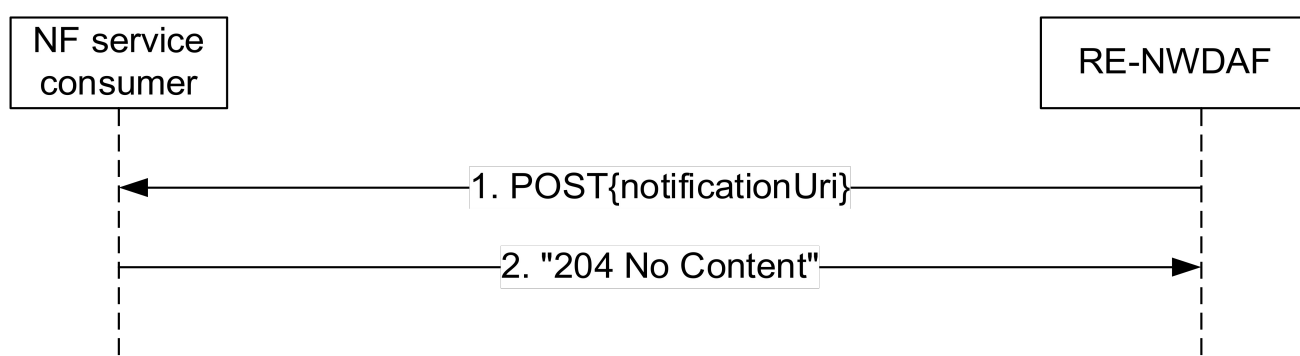
Figure 4.8.2.4.2-1: RE-NWDAF notifies the subscribed event
