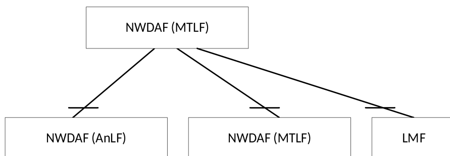
Figure 4.5.1.2-2: Reference Architecture for the Nnwdafl_MLModelProvision Service: reference point representation
