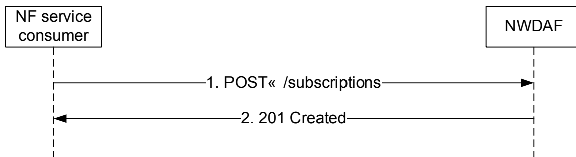
Figure 4.2.2.2.2-1: NF service consumer subscribes to notifications
