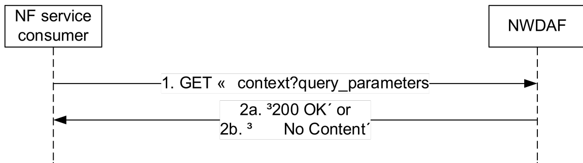
Figure 4.3.2.3.2-1: Requesting NWDAF context information related to analytics subscriptions
