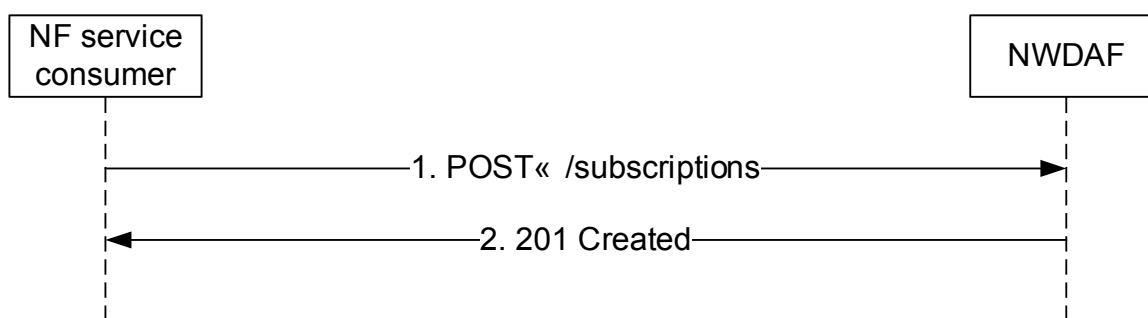
Figure 4.6.2.2.2-1: NF service consumer subscribes to notifications
