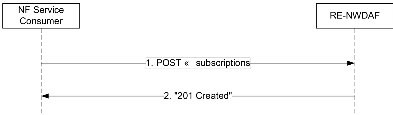
Figure 4.8.2.2.2-1: NF service consumer subscribes to notifications
