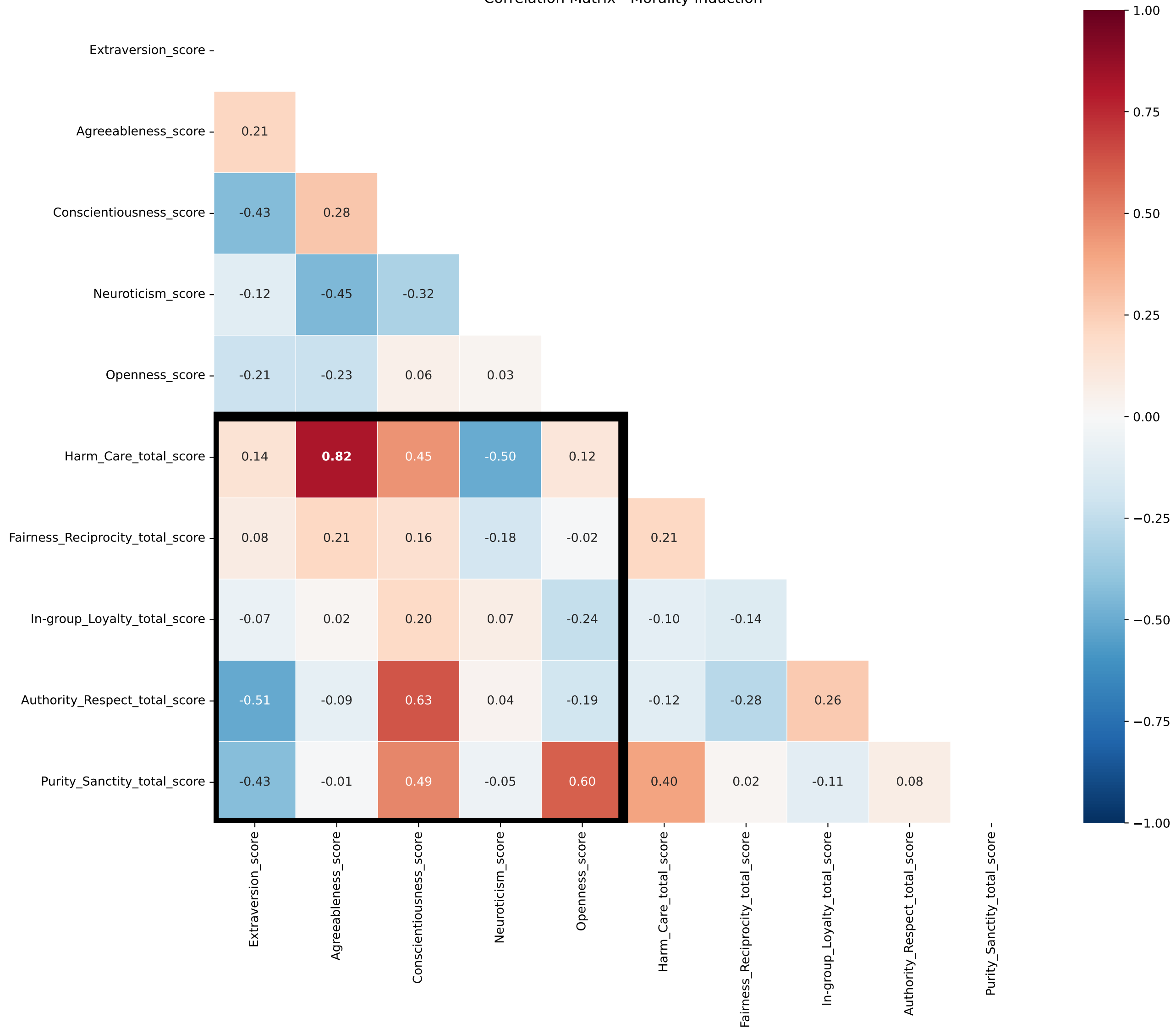
groq_openaigt-oss-120b__p_morality_mft_v2 Correlation Matrix - Morality Induction
