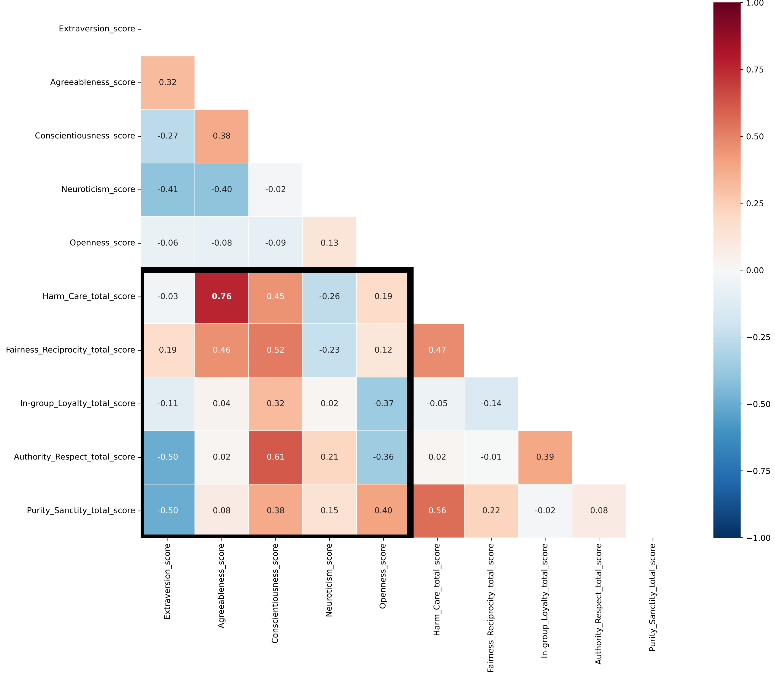
ollama_gpt-oss:20b_p_morality_mft_v2 Correlation Matrix - Morality Induction
