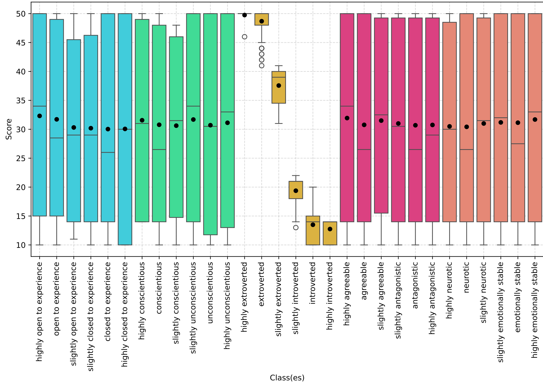
Score Distribution - Extraversion
