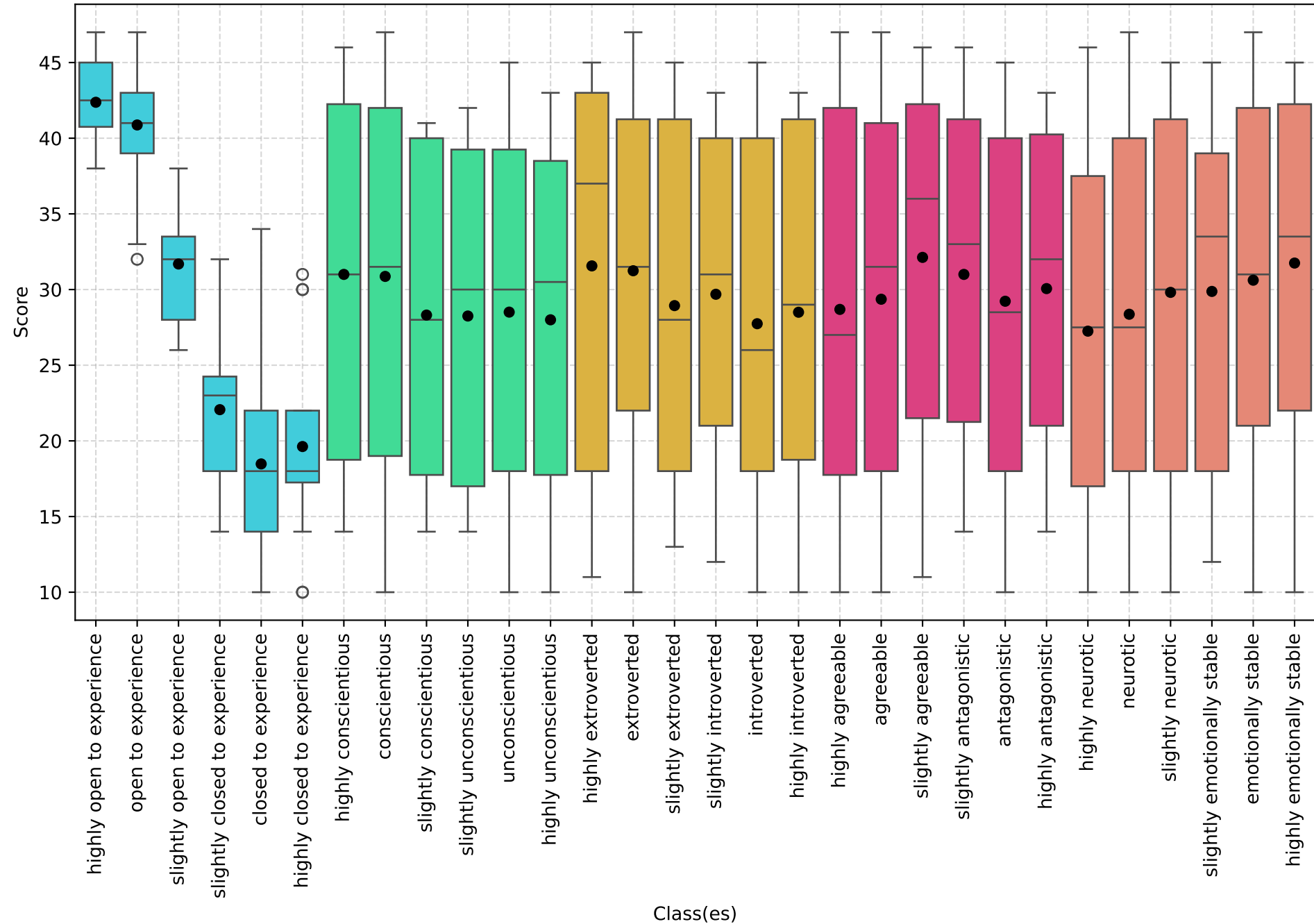
Score Distribution - Openness
