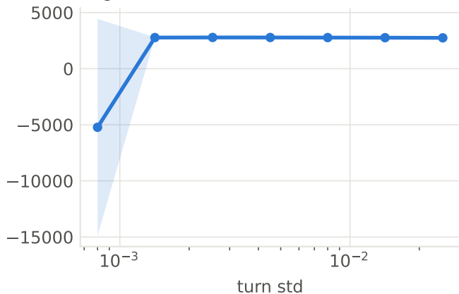
Log likelihood
