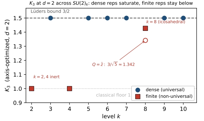
FIG. 1. K_3 at d = 2 (spin- \frac{1}{2} ) across SU(2)_k , axis-optimized reading. Dense levels k \in \{3, 5, 6, 7, 9, 10\} saturate the Lüders bound 3/2 ; the finite levels k \in \{2, 4, 8\} (minimal-rank, one-qubit space) stay strictly below— k = 2, 4 at the classical floor 1, and k = 8 at 1.427 (its Q = \hat{z} reading 3/\sqrt{5} \approx 1.342 is the open marker). The closest finite representation, k = 8 , sits only \approx 0.07 below the bound.
