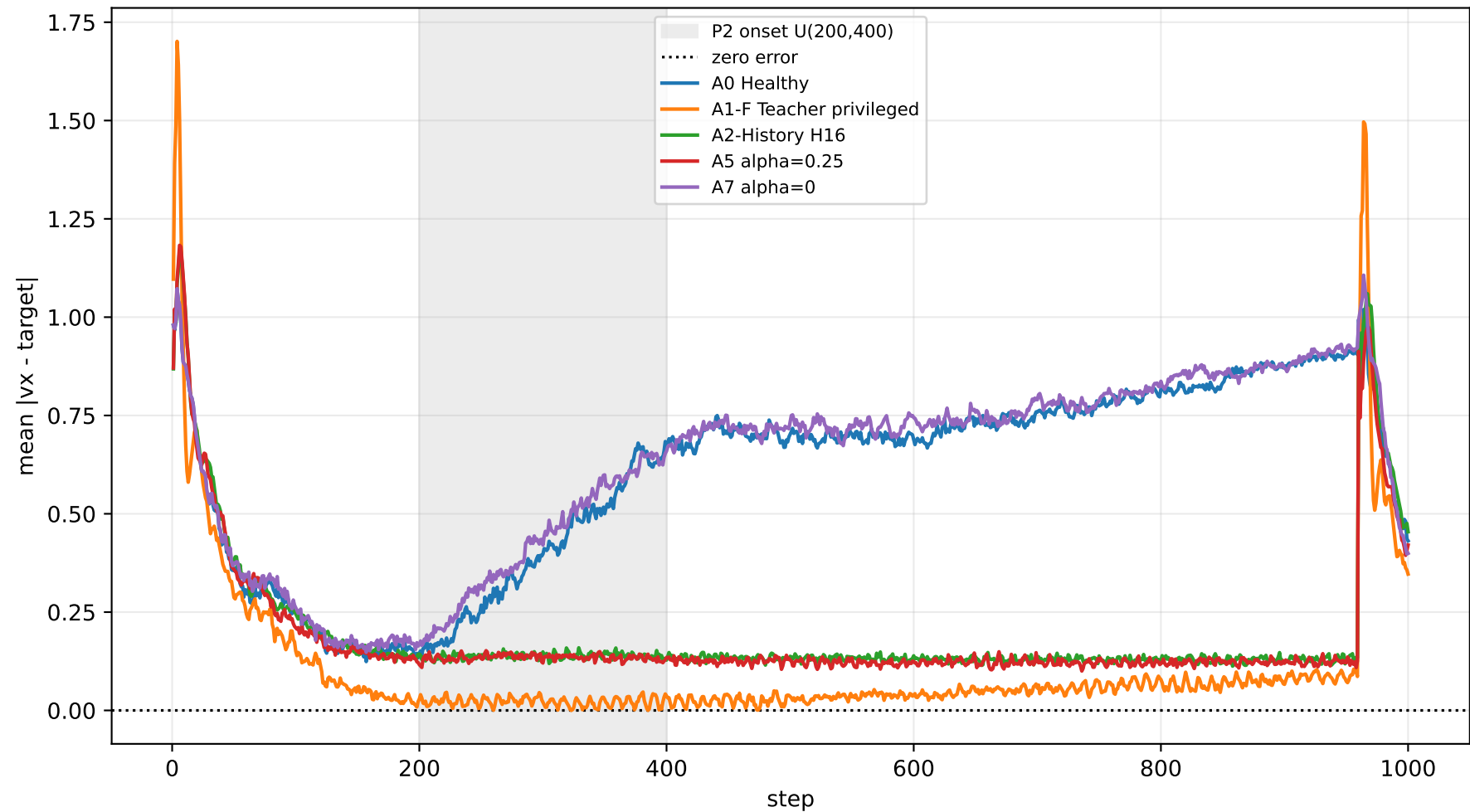
T12 random onset: absolute vx error over time
