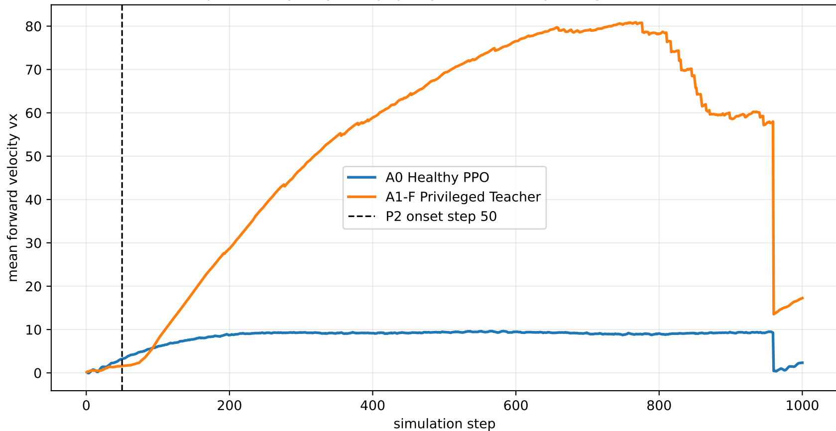
Quick P2 Sanity Demo: Forward Velocity Before/After Joint Lock quick sanity only, not paper-grade; A1-F is privileged teacher
