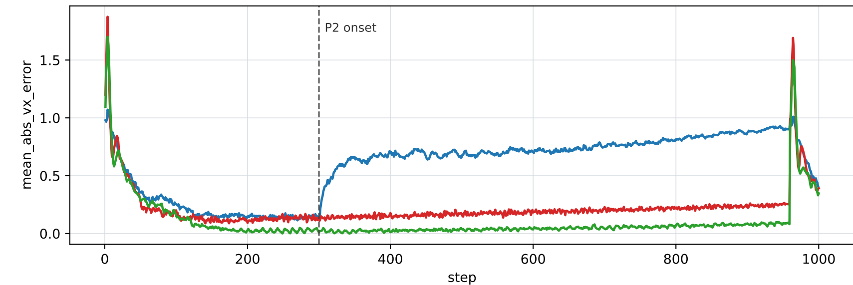
Velocity tracking error after settled-regime P2 fault
