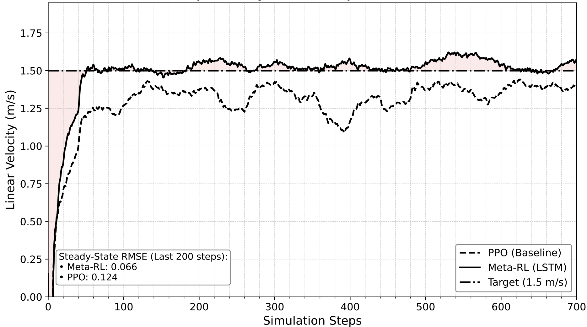
Velocity Tracking under Heavy Load (3.0x Mass)
