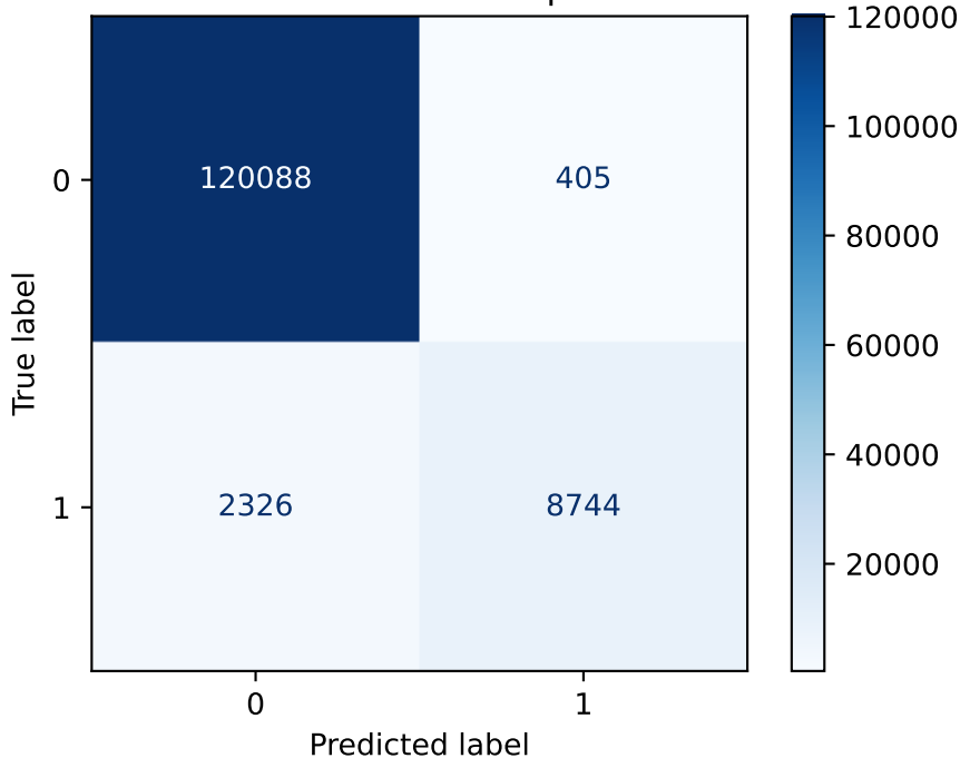
Confusion Matrix: Deeper tree
