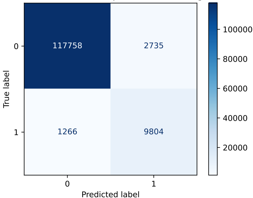
Confusion Matrix: Deep tree & more weight
