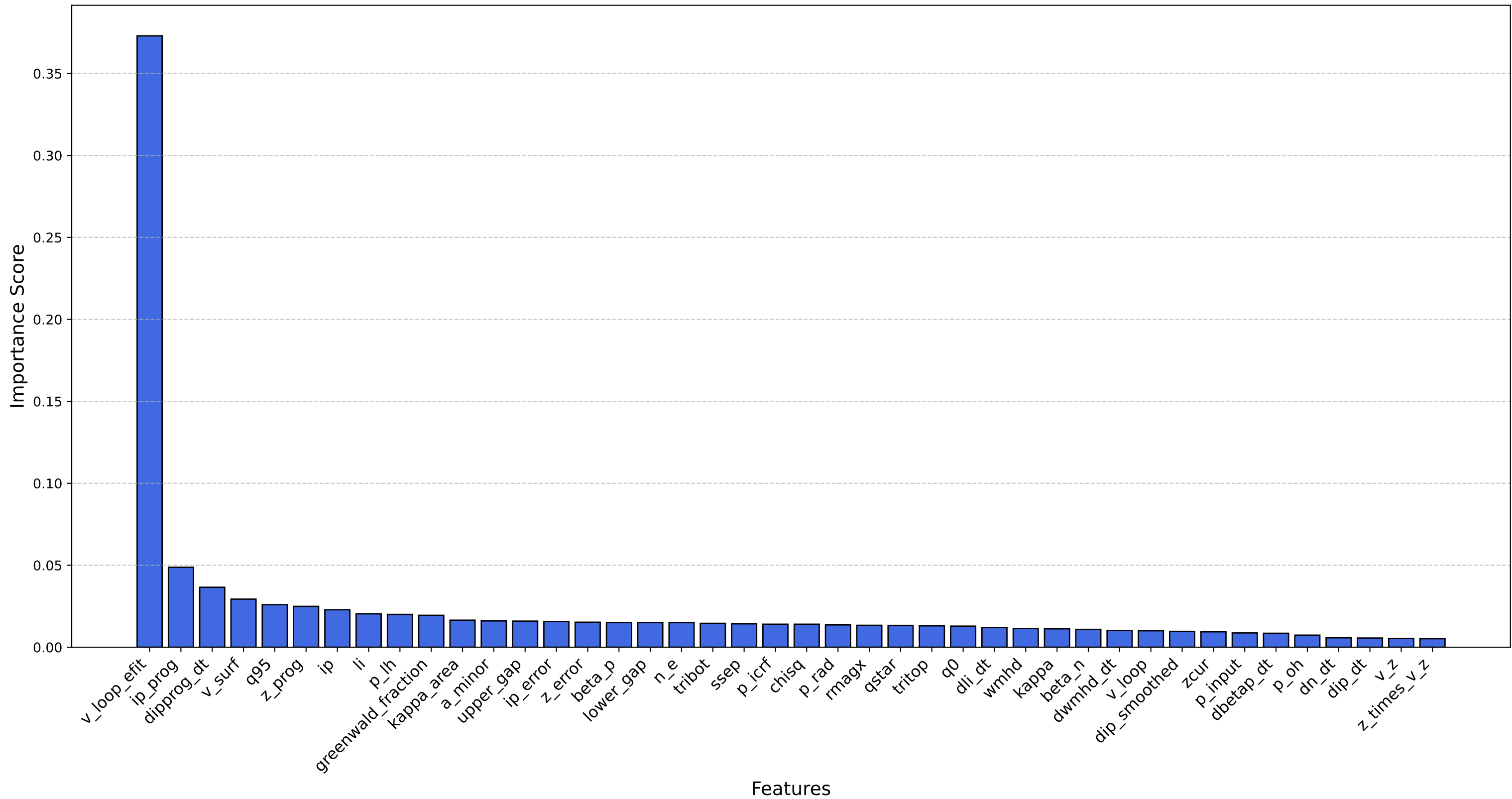
XGBoost Model - Feature Importances (Deep Tree & More Weight)
