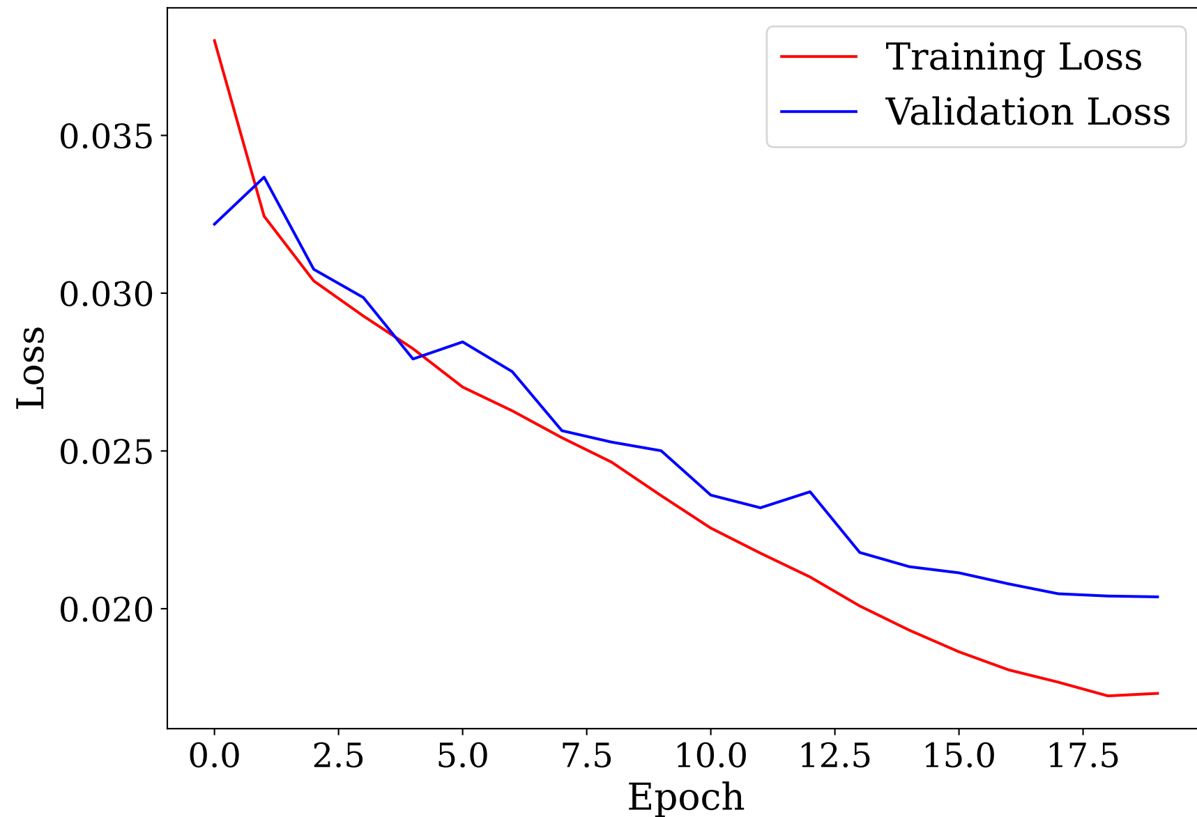
Bounded Values
