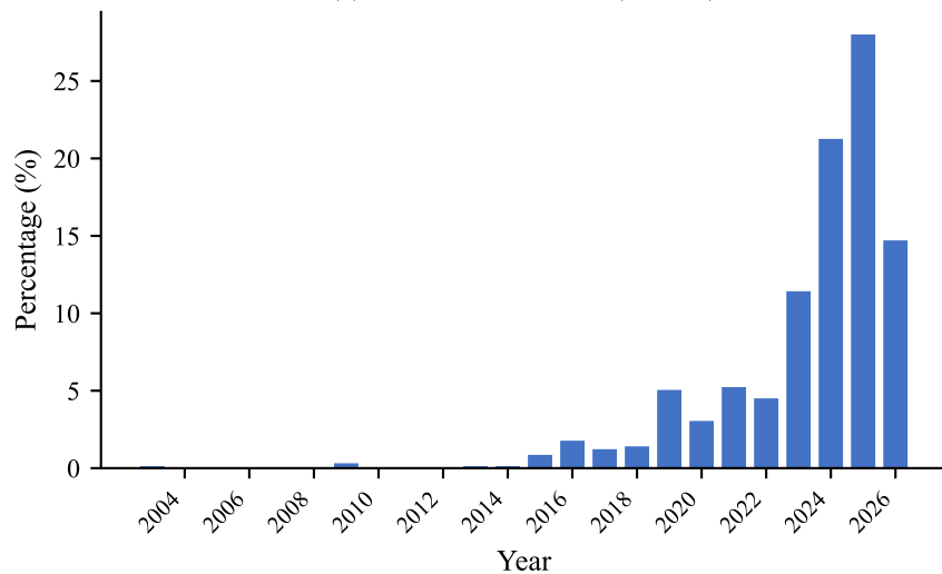
(c) Publication Year (n=549)
