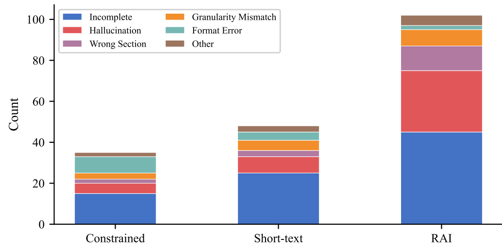
(b) Failure Modes by Field Type
