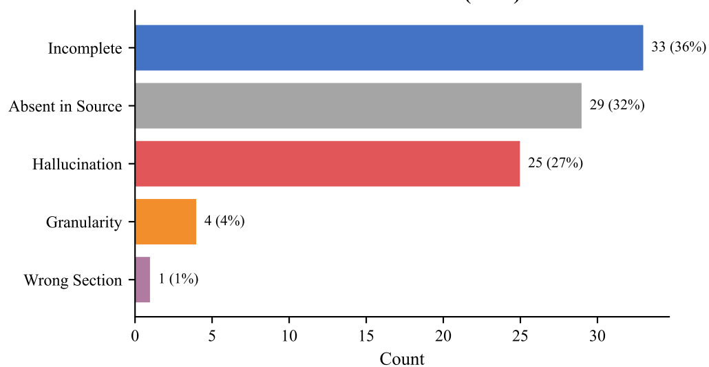
Overall Distribution (n=92)
