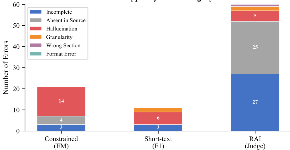
Error Types by Field Category
