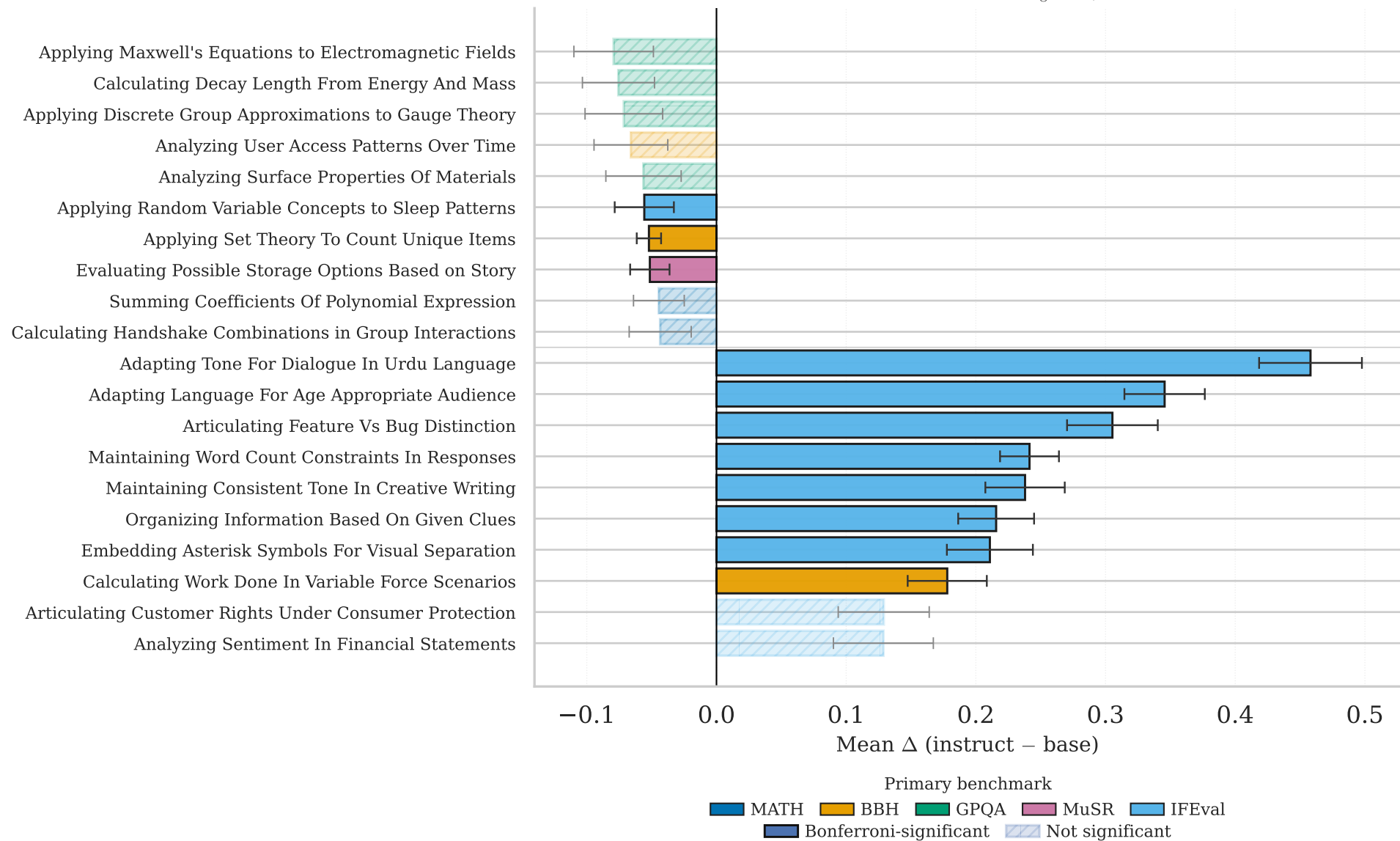
(b) Top-10 improved and degraded skills ( n_{\text{Bonf-sig}} = 14/100 across all skills)
