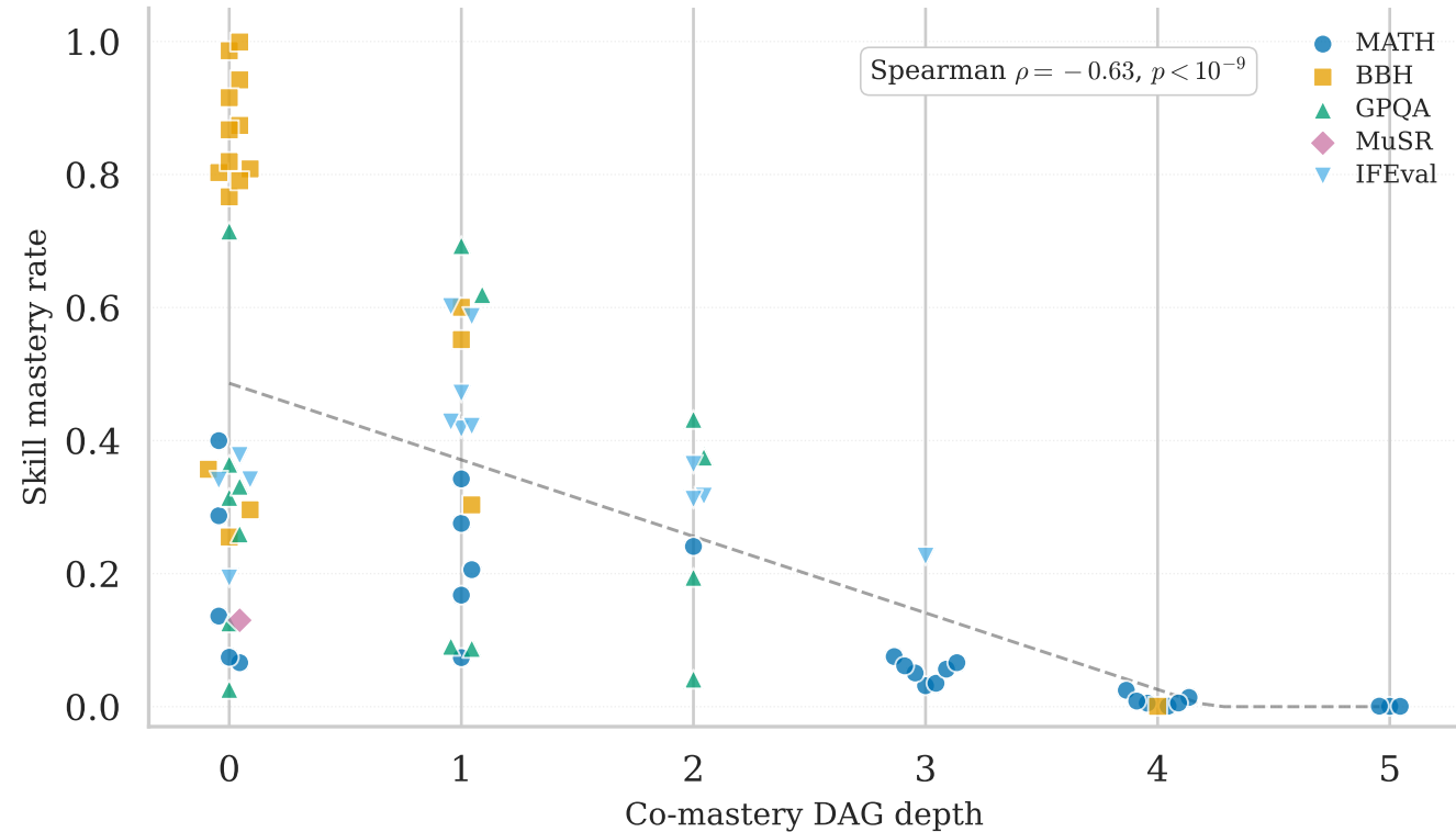
(a) Per-skill mastery by depth
