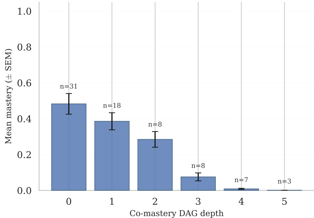
(b) Mean mastery per depth level
