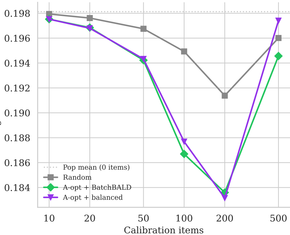
RMSE vs ground-truth theta
