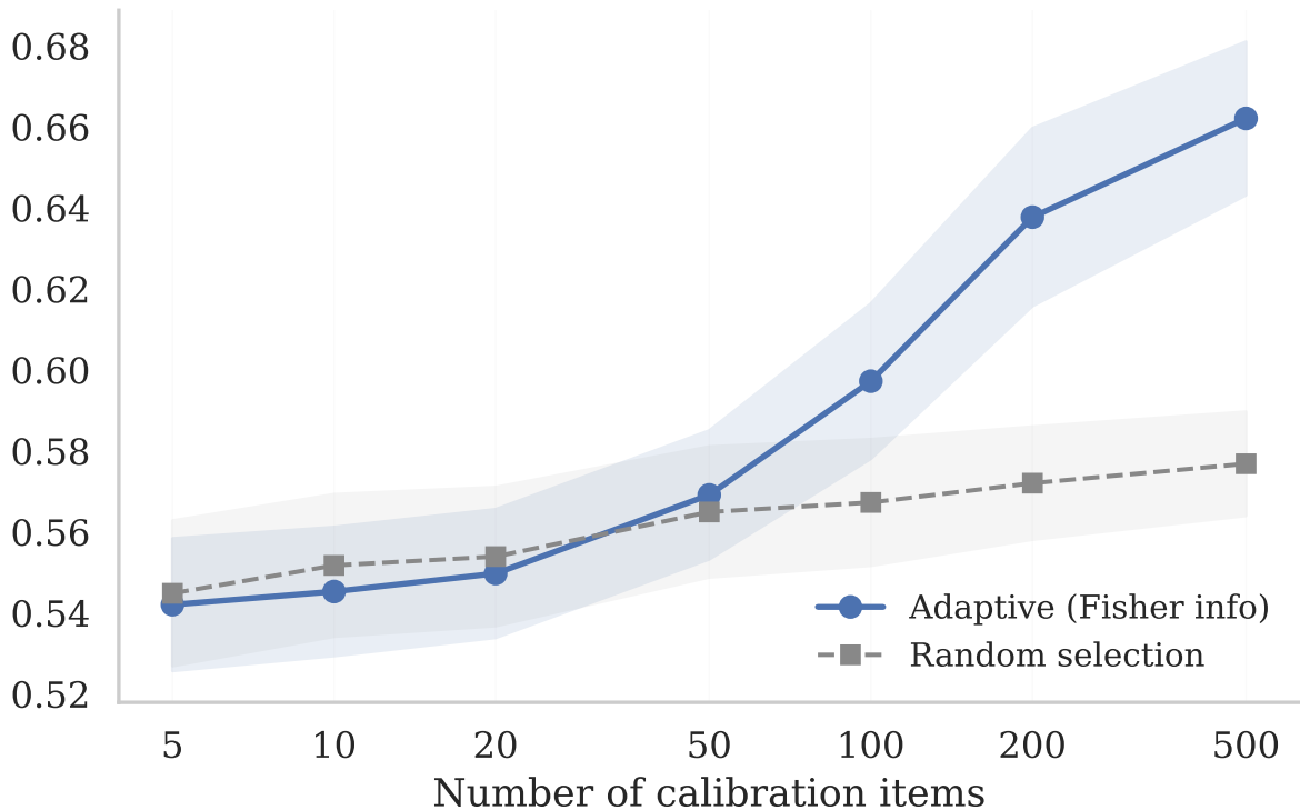
AUC on held-out test items
