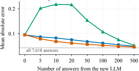
(a) Predicting benchmark scores (lower is better)
