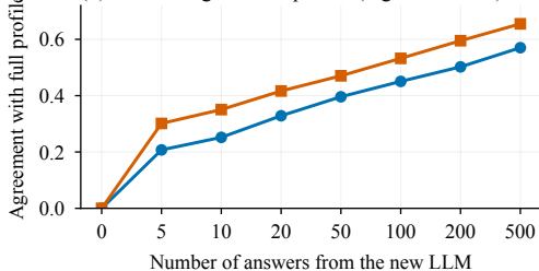
(b) Recovering the skill profile (higher is better)
