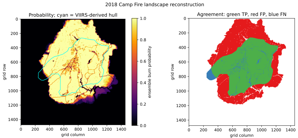
Figure 5: Ensemble burn probability, VIIRS-derived support, and cell-level true-positive, false-positive, and false-negative regions.
