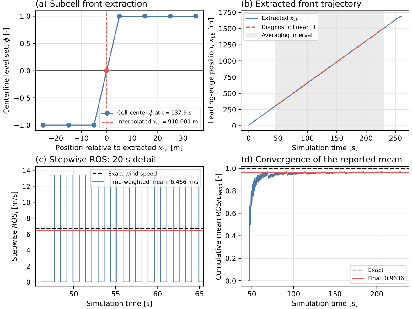
Figure 4: Detailed extraction for the representative \Delta x = 10 m, CFL_{wind} = 0.5 simulation. (a) Linear interpolation of centerline \phi = 0 crossings; (b) resulting leading-edge trajectory and diagnostic fit; (c) a 20-second zoom of consecutive-dump finite-difference ROS and its time-weighted mean; (d) convergence of the cumulative normalized mean to its reported value.
