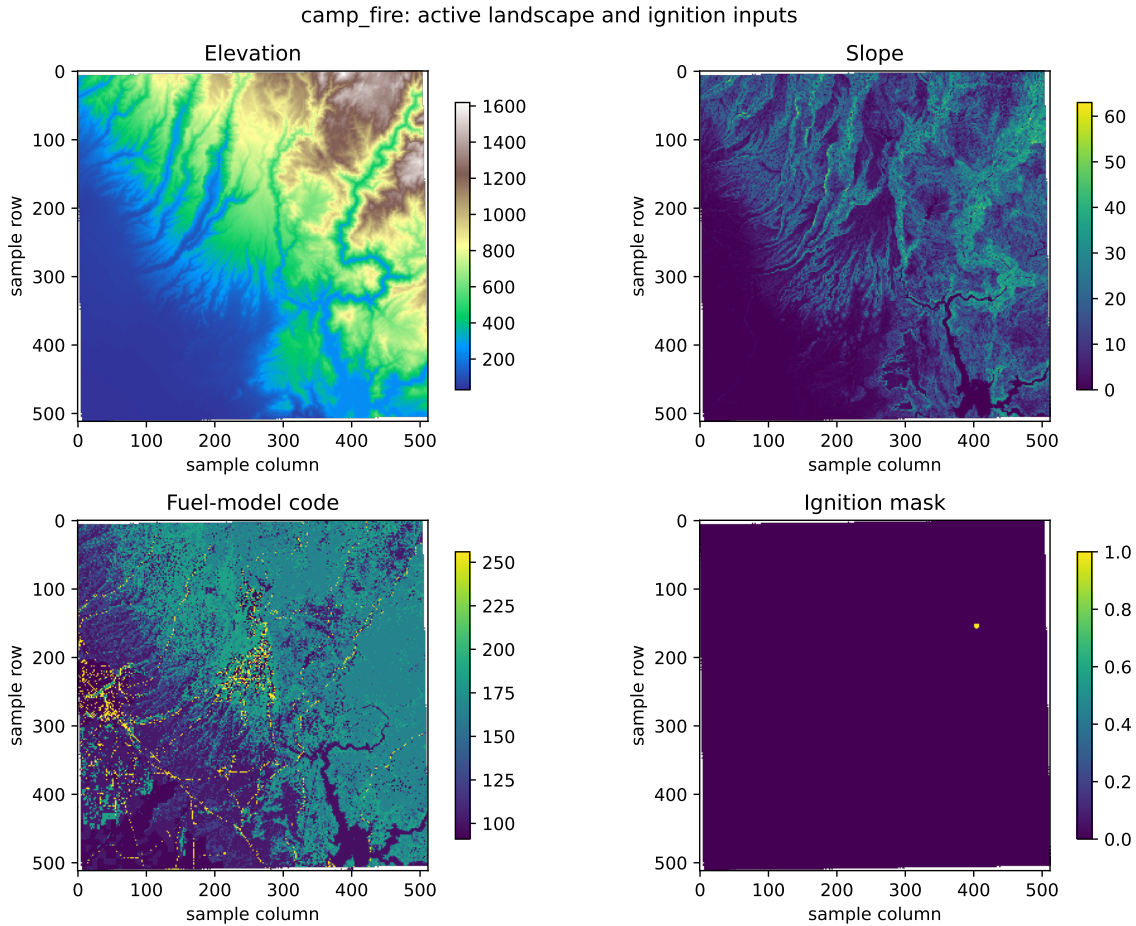
Figure 2: Active elevation, slope, fuel-model, and ignition-mask inputs. These plots characterize model forcing; they are not validation evidence.
