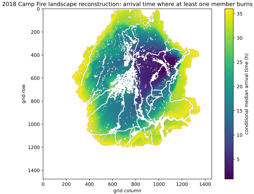
Figure 6: Conditional median arrival time among members that burn each cell by the comparison time. Conditioning is stated because it omits no-burn members.
