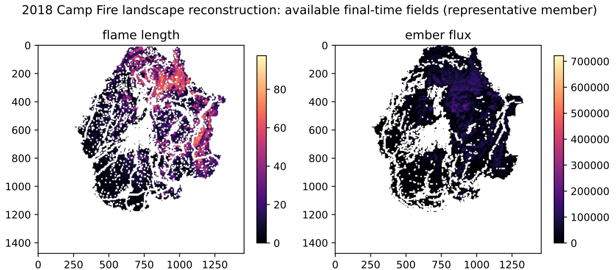
Figure 7: Applicable final-time two-dimensional fields found by the postprocessor. Omission of this panel means no recognized optional field was available; it does not imply a zero field.
