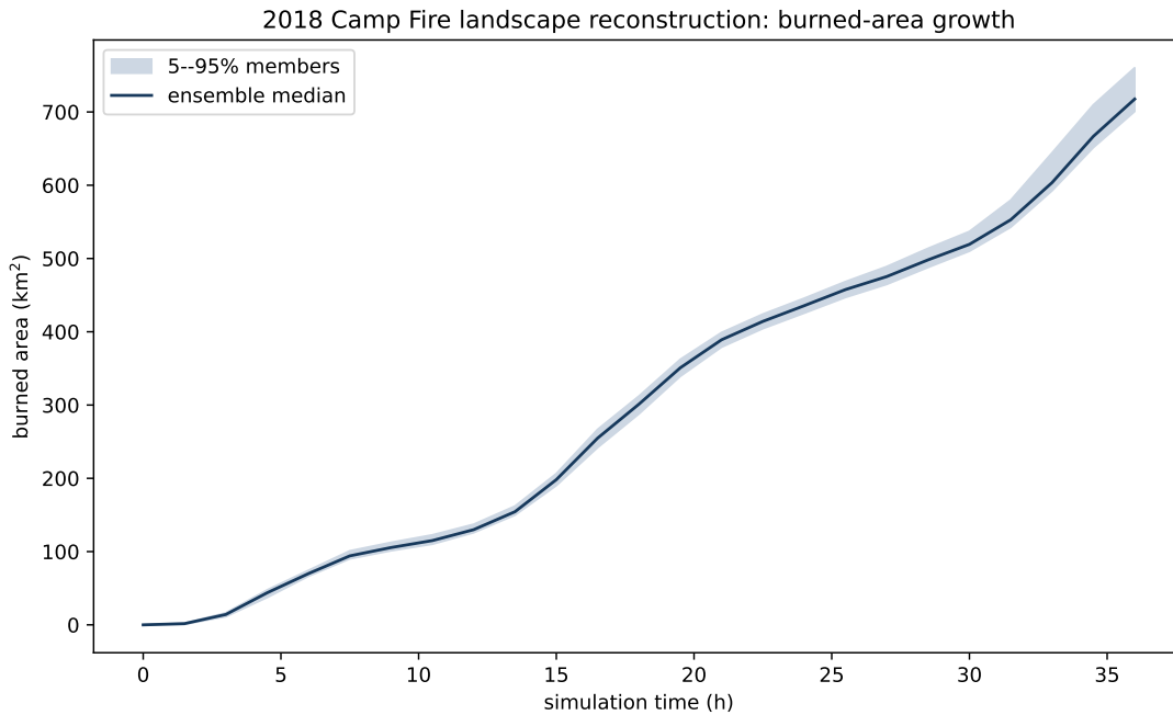
Figure 8: Median and 5th–95th percentile ensemble burned-area growth.
