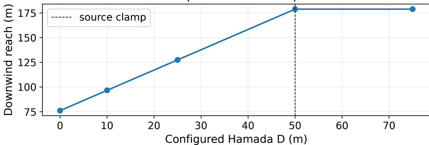
Separation and clamp
