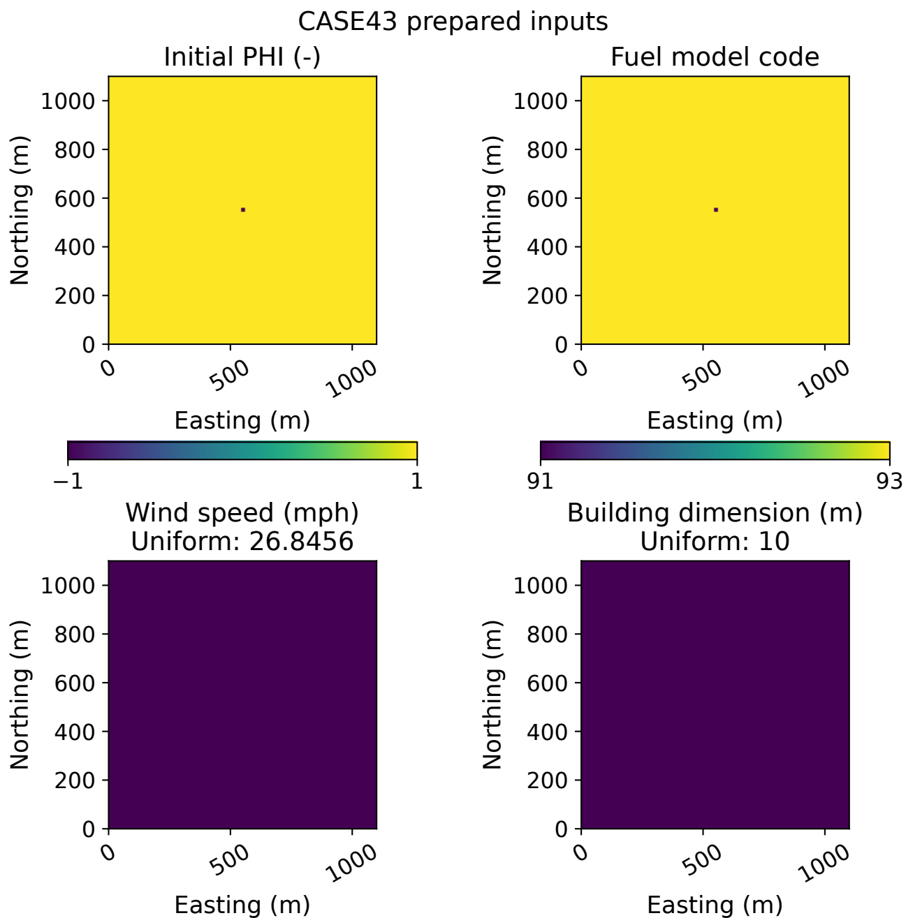
Figure 2: Whole-domain prepared configuration generated from the rotation_wd270 GeoTIFF inputs. The single negative PHI cell is the initial WU-E source; FBFM93 and zero adjustment prevent secondary spread.
