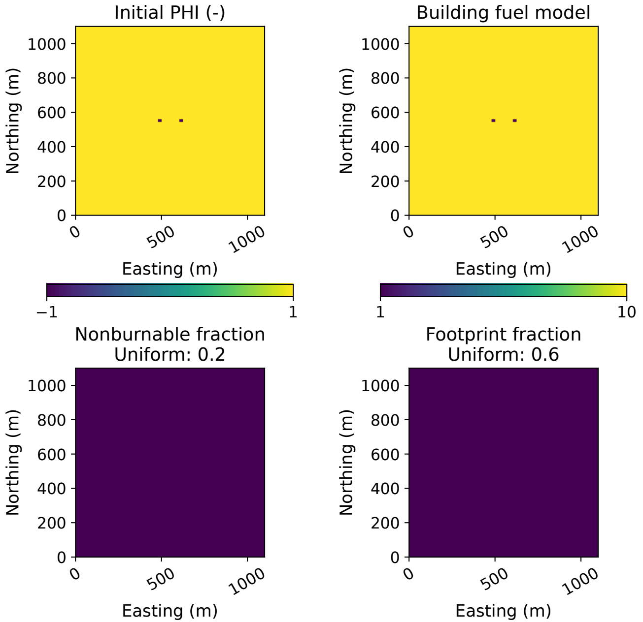
Figure 2: Prepared two-source configuration read back from generated GeoTIFFs. Source model IDs override the uniform target-table ID only at the two initially burning cells.
