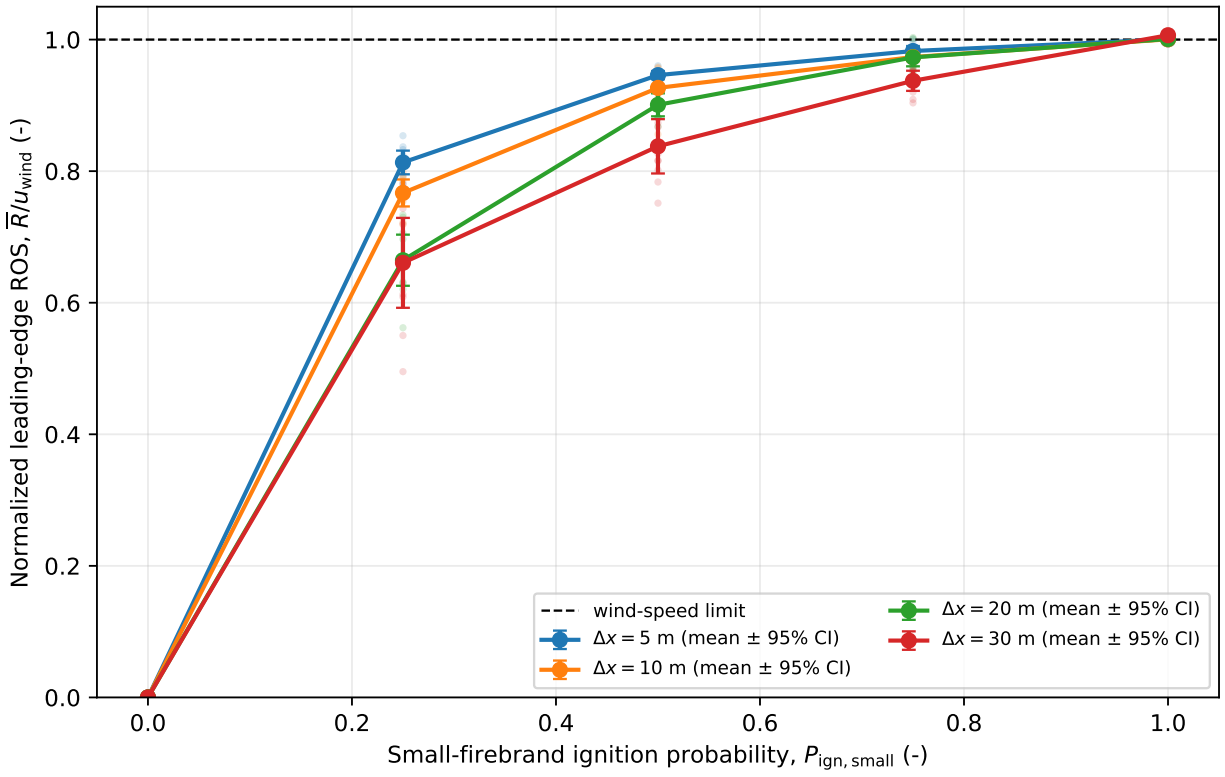
Figure 4: Ensemble-mean normalized leading-edge ROS versus P_{ign, small} . Error bars are 95% confidence intervals and faint points are independently seeded ELMFIRE members.
