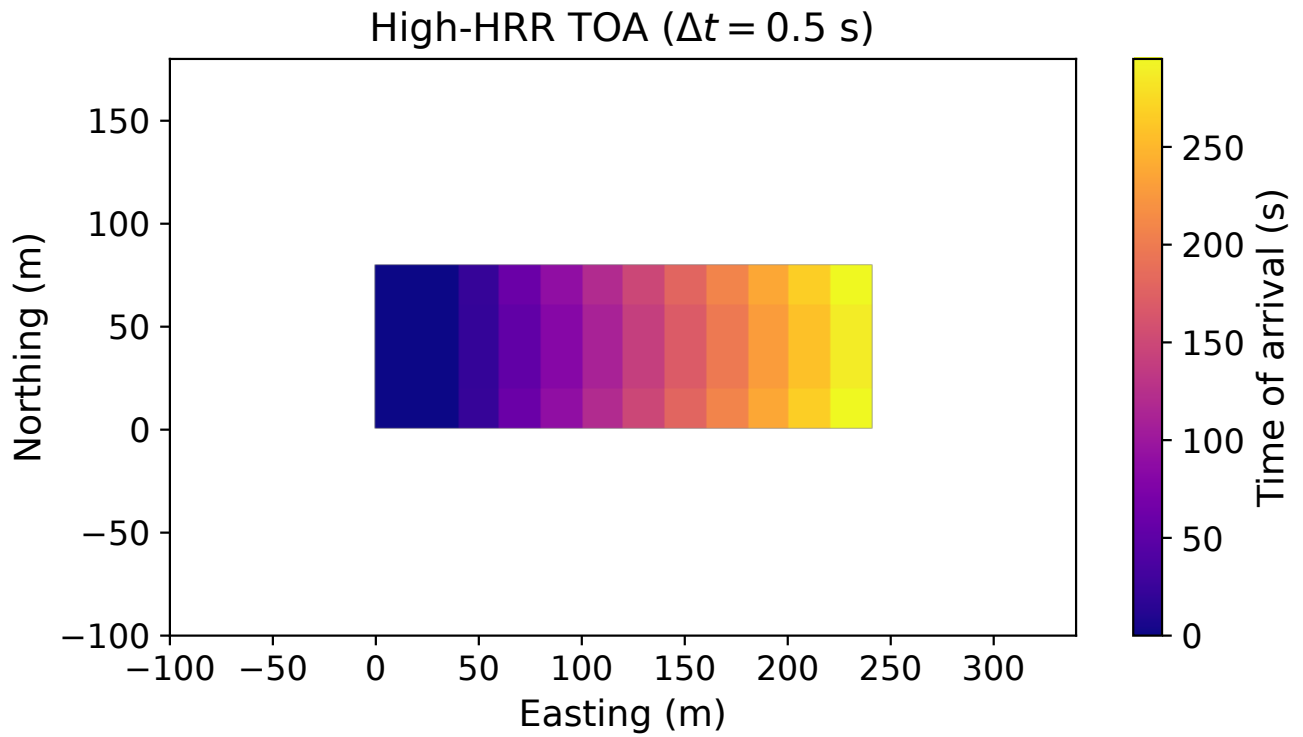
Figure 3: High-HRR exact- t = 300 s TOA for \Delta t = 0.5 s; the exact source raster is recorded in outputs/metrics.json .
