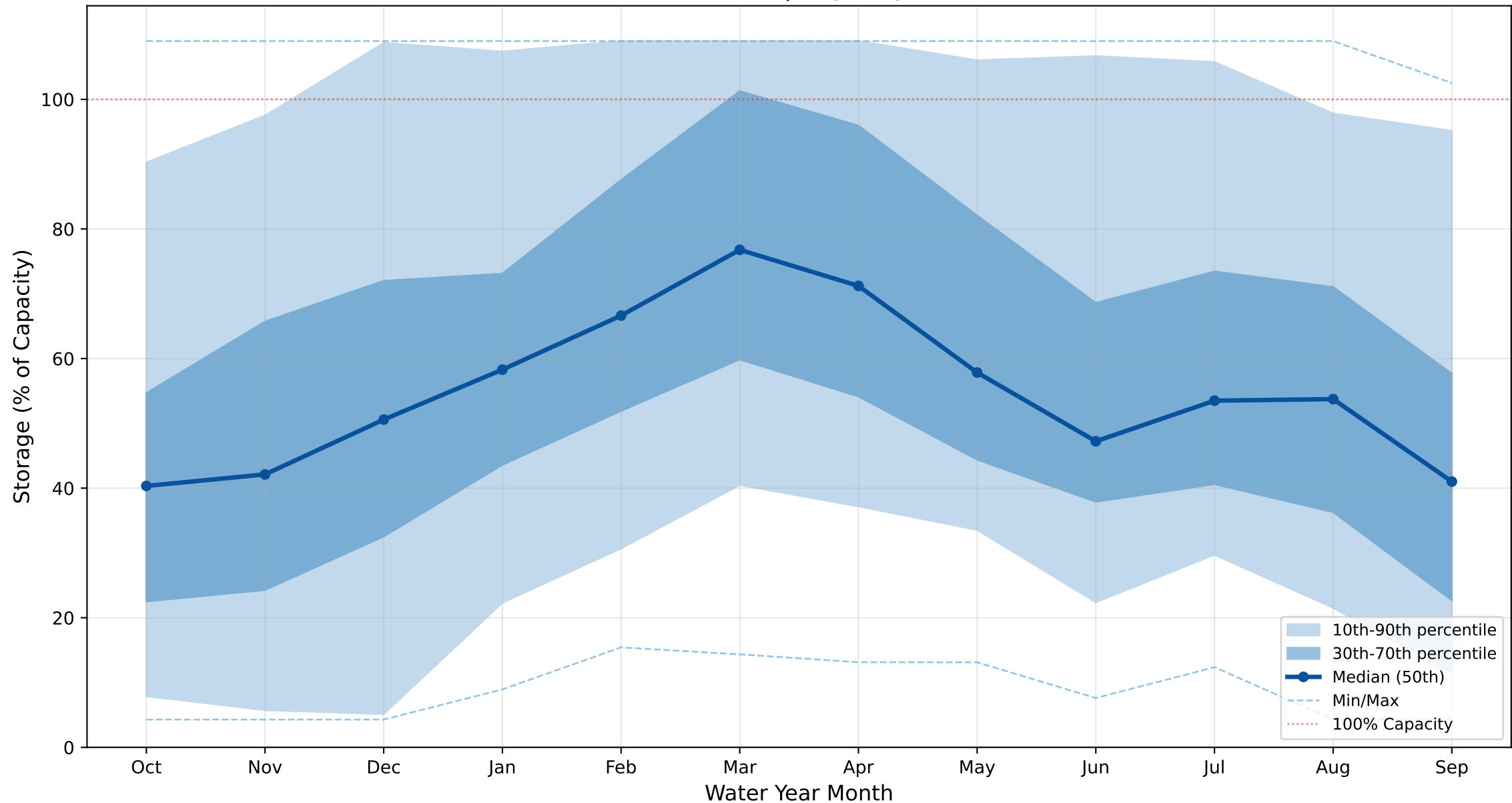
San Luis SWP (SLUIS_SWP) - Monthly Storage Percentiles Scenario: s0020 | Capacity: 979 TAF
