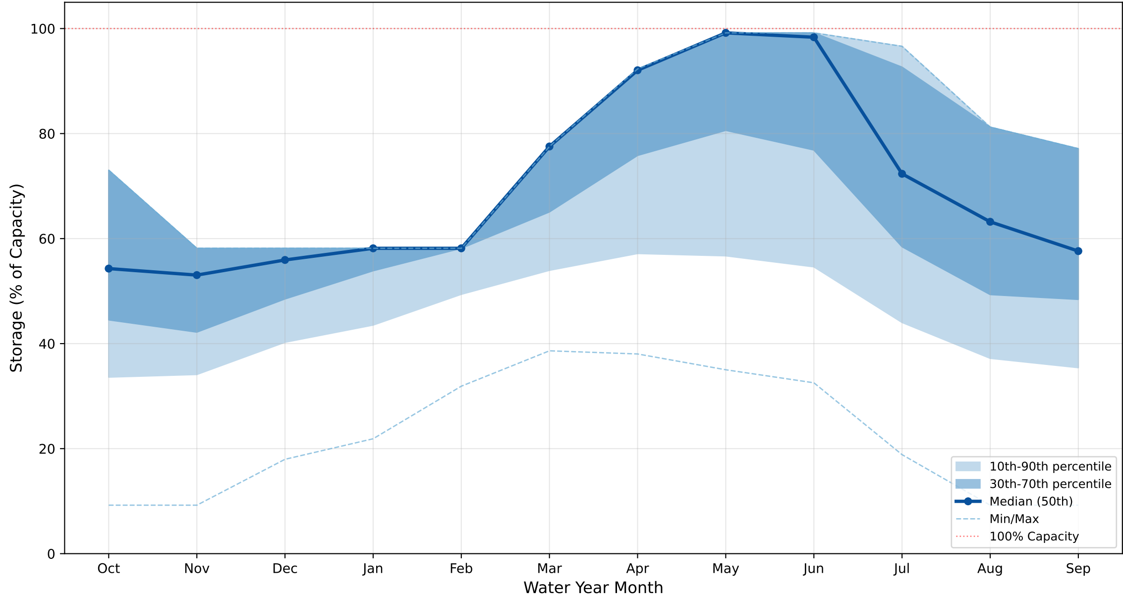
Folsom (FOLSM) - Monthly Storage Percentiles Scenario: s0020 | Capacity: 975 TAF
