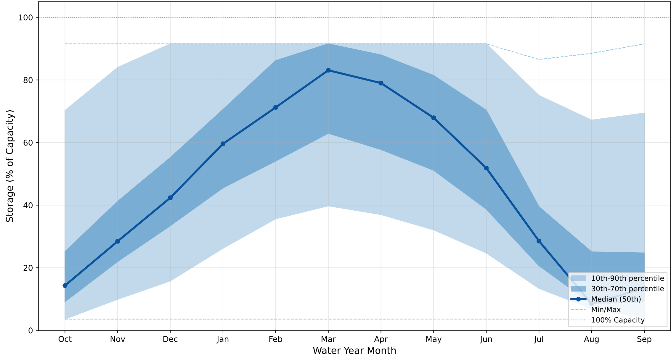
San Luis CVP (SLUIS_CVP) - Monthly Storage Percentiles Scenario: s0020 | Capacity: 1,062 TAF
