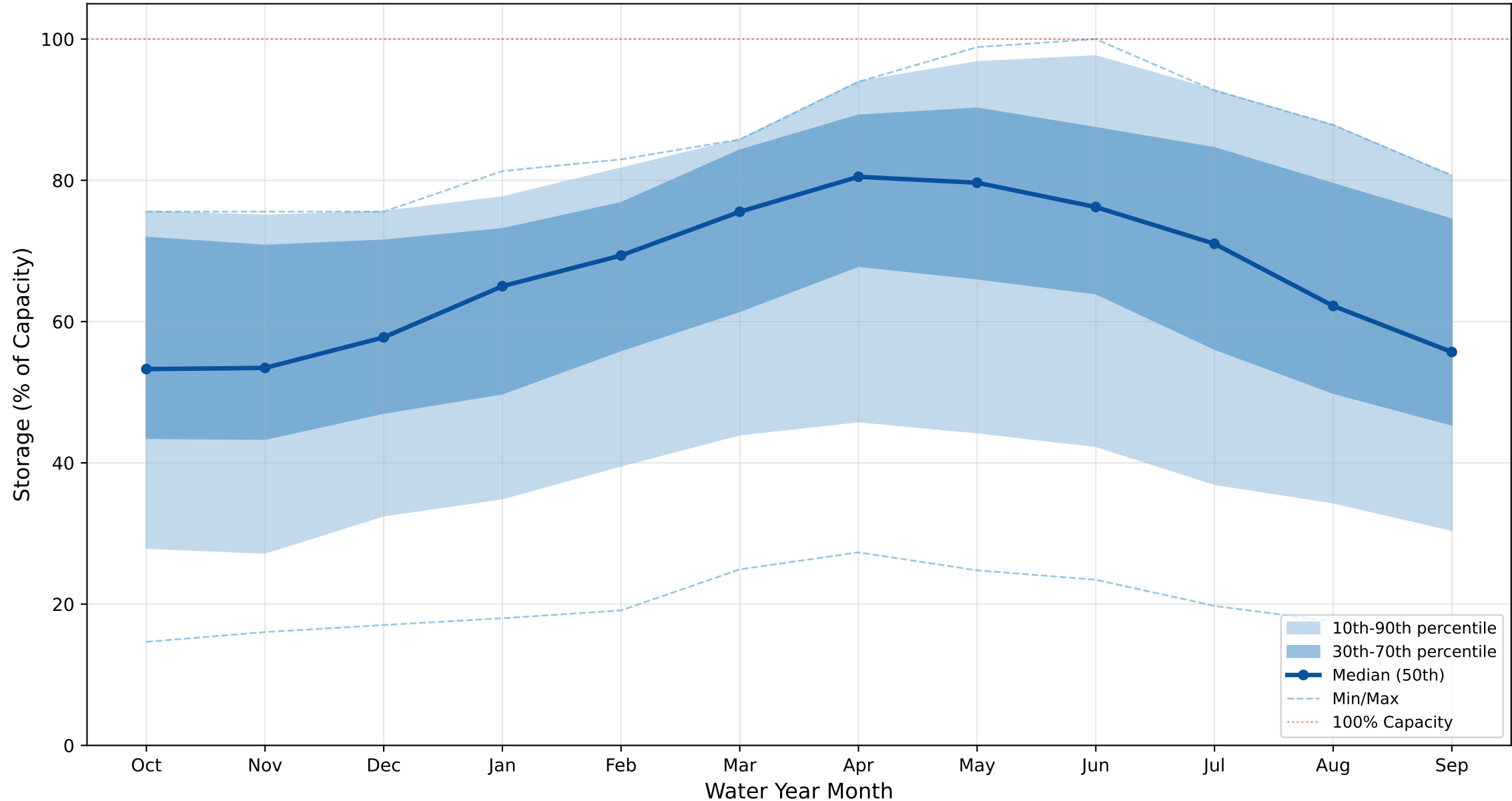
Trinity (TRNTY) - Monthly Storage Percentiles Scenario: s0020 | Capacity: 2,448 TAF
