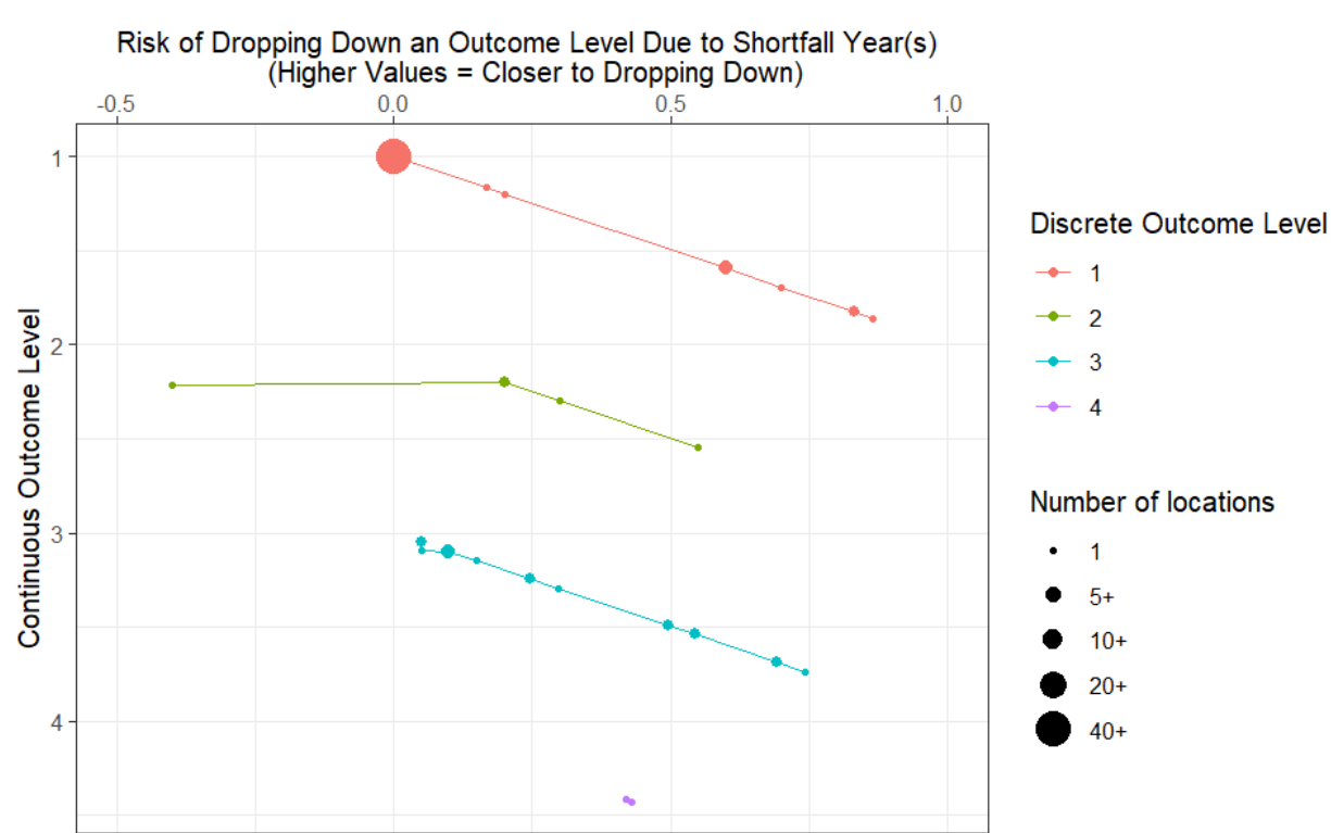
Figure 6. Severity drop risk across discrete and continuous outcome level values for locations of interest in the baseline scenario (s0020). Severity drop risk = (1 - \text{normalized severity score}) \times 0.99 .
