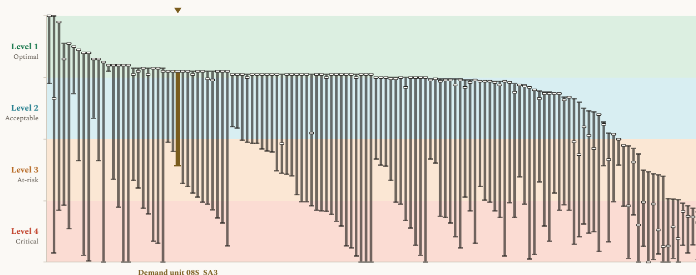
Figure 2. Revenue results, presented as modeled outcome levels, across the 132 agricultural revenue locations, with Demand unit 08S_SA3 marked. Each column shows the span of modeled results for one agricultural water service area across the COEQWAL library. Ends of a column are the lowest and the highest modeled value at that location across the runs that report it. A short dash across a column is that location's own baseline (current operations under the historical hydroclimate). This figure uses the same value axis (y-axis) format as Figure 1. Every column uses the same encoding; the column for Demand unit 08S_SA3, this brief's subject, is drawn wider, in a distinct color, and marked above. The scale is set out in how to read the values.
