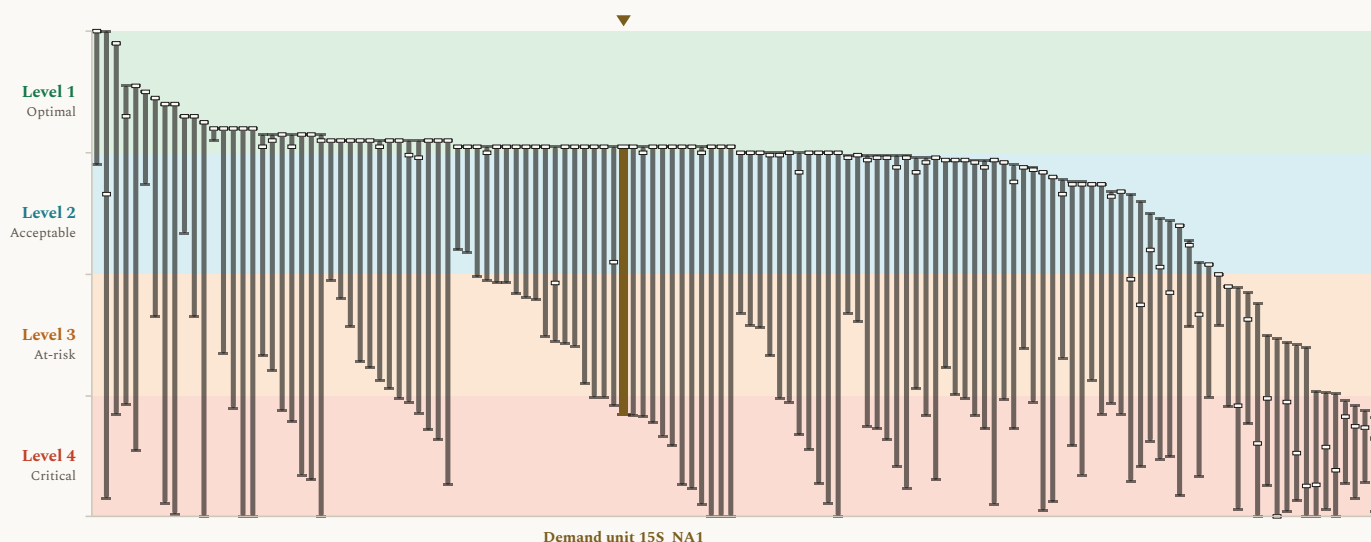
Figure 2. Revenue results, presented as modeled outcome levels, across the 132 agricultural revenue locations, with Demand unit 15S_NA1 marked. Each column shows the span of modeled results for one agricultural water service area across the COEQWAL library. Ends of a column are the lowest and the highest modeled value at that location across the runs that report it. A short dash across a column is that location's own baseline (current operations under the historical hydroclimate). This figure uses the same value axis (y-axis) format as Figure 1. Every column uses the same encoding; the column for Demand unit 15S_NA1, this brief's subject, is drawn wider, in a distinct color, and marked above. The scale is set out in how to read the values.
