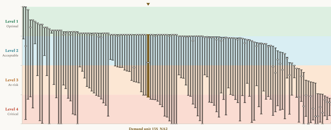
Figure 2. Revenue results, presented as modeled outcome levels, across the 132 agricultural revenue locations, with Demand unit 15S_NA2 marked. Each column shows the span of modeled results for one agricultural water service area across the COEQWAL library. Ends of a column are the lowest and the highest modeled value at that location across the runs that report it. A short dash across a column is that location's own baseline (current operations under the historical hydroclimate). This figure uses the same value axis (y-axis) format as Figure 1. Every column uses the same encoding; the column for Demand unit 15S_NA2, this brief's subject, is drawn wider, in a distinct color, and marked above. The scale is set out in how to read the values.
