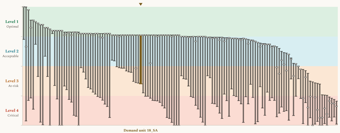
Figure 2. Revenue results, presented as modeled outcome levels, across the 132 agricultural revenue locations, with Demand unit 18_SA marked. Each column shows the span of modeled results for one agricultural water service area across the COEQWAL library. Ends of a column are the lowest and the highest modeled value at that location across the runs that report it. A short dash across a column is that location's own baseline (current operations under the historical hydroclimate). This figure uses the same value axis (y-axis) format as Figure 1. Every column uses the same encoding; the column for Demand unit 18_SA, this brief's subject, is drawn wider, in a distinct color, and marked above. The scale is set out in how to read the values.
