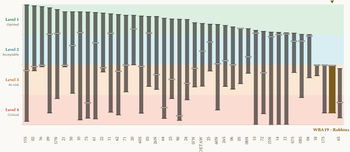
Figure 2. Groundwater storage results, presented as modeled outcome levels, across the 42 groundwater storage locations, with WBA19 - Robbins marked. Each column shows the span of modeled results for one groundwater basin area across the COEQWAL library. Ends of a column are the lowest and the highest modeled value at that location across the runs that report it. A short dash across a column is that location's own baseline (current operations under the historical hydroclimate). This figure uses the same value axis (y-axis) format as Figure 1. Every column uses the same encoding; the column for WBA19 - Robbins, this brief's subject, is drawn wider, in a distinct color, and marked above. The scale is set out in how to read the values.
