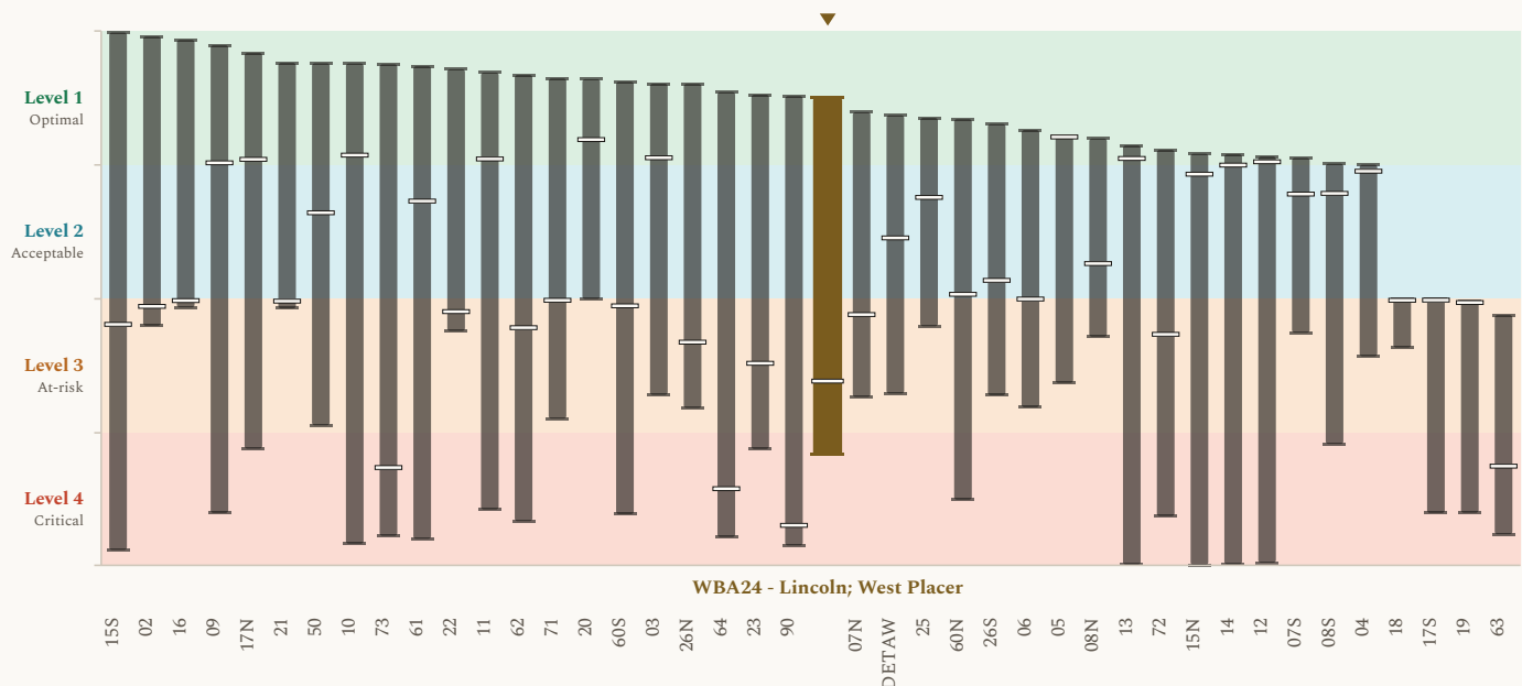
Figure 2. Groundwater storage results, presented as modeled outcome levels, across the 42 groundwater storage locations, with WBA24 - Lincoln; West Placer marked. Each column shows the span of modeled results for one groundwater basin area across the COEQWAL library. Ends of a column are the lowest and the highest modeled value at that location across the runs that report it. A short dash across a column is that location's own baseline (current operations under the historical hydroclimate). This figure uses the same value axis (y-axis) format as Figure 1. Every column uses the same encoding; the column for WBA24 - Lincoln; West Placer, this brief's subject, is drawn wider, in a distinct color, and marked above. The scale is set out in how to read the values.
