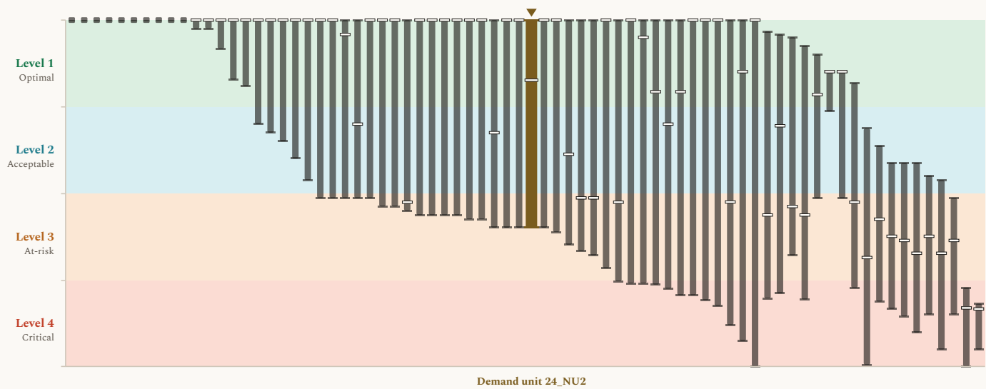
Figure 2. Delivery results, presented as modeled outcome levels, across the 74 community surface water locations, with Demand unit 24_NU2 marked. Each column shows the span of modeled results for one community water system across the COEQWAL library. Ends of a column are the lowest and the highest modeled value at that location across the runs that report it. A short dash across a column is that location's own baseline (current operations under the historical hydroclimate). This figure uses the same value axis (y-axis) format as Figure 1. Every column uses the same encoding; the column for Demand unit 24_NU2, this brief's subject, is drawn wider, in a distinct color, and marked above. The scale is set out in how to read the values.
