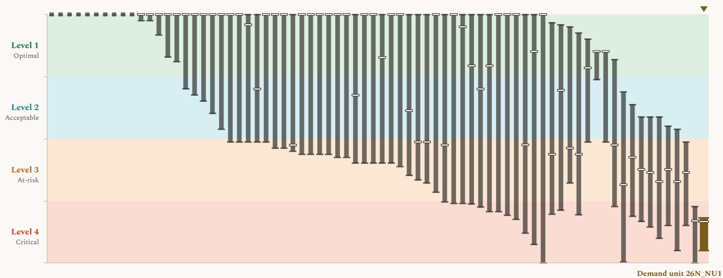
Figure 2. Delivery results, presented as modeled outcome levels, across the 74 community surface water locations, with Demand unit 26N_NU1 marked. Each column shows the span of modeled results for one community water system across the COEQWAL library. Ends of a column are the lowest and the highest modeled value at that location across the runs that report it. A short dash across a column is that location's own baseline (current operations under the historical hydroclimate). This figure uses the same value axis (y-axis) format as Figure 1. Every column uses the same encoding; the column for Demand unit 26N_NU1, this brief's subject, is drawn wider, in a distinct color, and marked above. The scale is set out in how to read the values.
