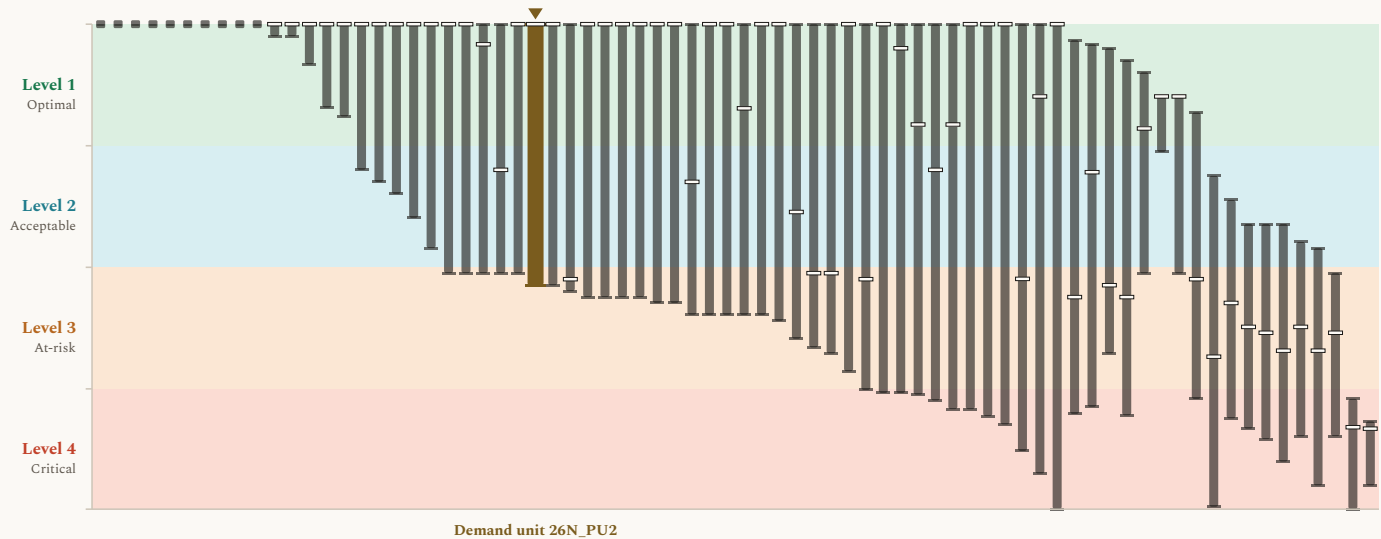
Figure 2. Delivery results, presented as modeled outcome levels, across the 74 community surface water locations, with Demand unit 26N_PU2 marked. Each column shows the span of modeled results for one community water system across the COEQWAL library. Ends of a column are the lowest and the highest modeled value at that location across the runs that report it. A short dash across a column is that location's own baseline (current operations under the historical hydroclimate). This figure uses the same value axis (y-axis) format as Figure 1. Every column uses the same encoding; the column for Demand unit 26N_PU2, this brief's subject, is drawn wider, in a distinct color, and marked above. The scale is set out in how to read the values.
