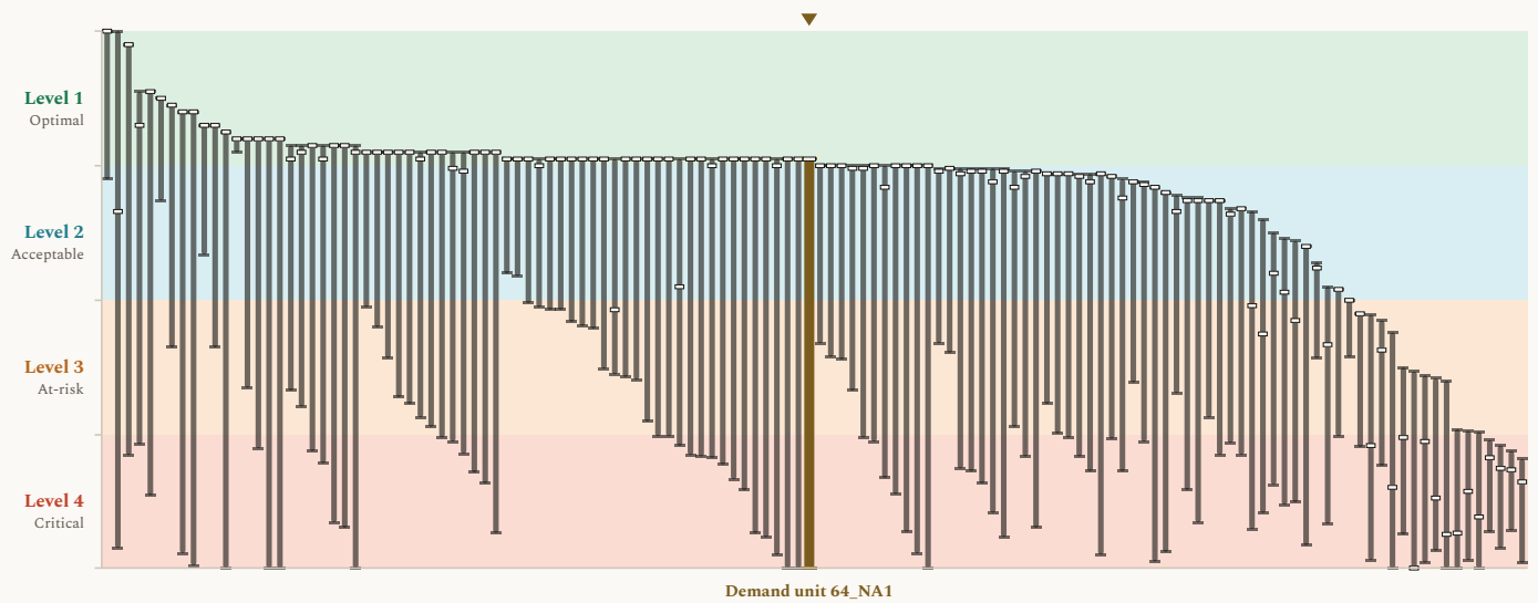
Figure 2. Revenue results, presented as modeled outcome levels, across the 132 agricultural revenue locations, with Demand unit 64_NA1 marked. Each column shows the span of modeled results for one agricultural water service area across the COEQWAL library. Ends of a column are the lowest and the highest modeled value at that location across the runs that report it. A short dash across a column is that location's own baseline (current operations under the historical hydroclimate). This figure uses the same value axis (y-axis) format as Figure 1. Every column uses the same encoding; the column for Demand unit 64_NA1, this brief's subject, is drawn wider, in a distinct color, and marked above. The scale is set out in how to read the values.
