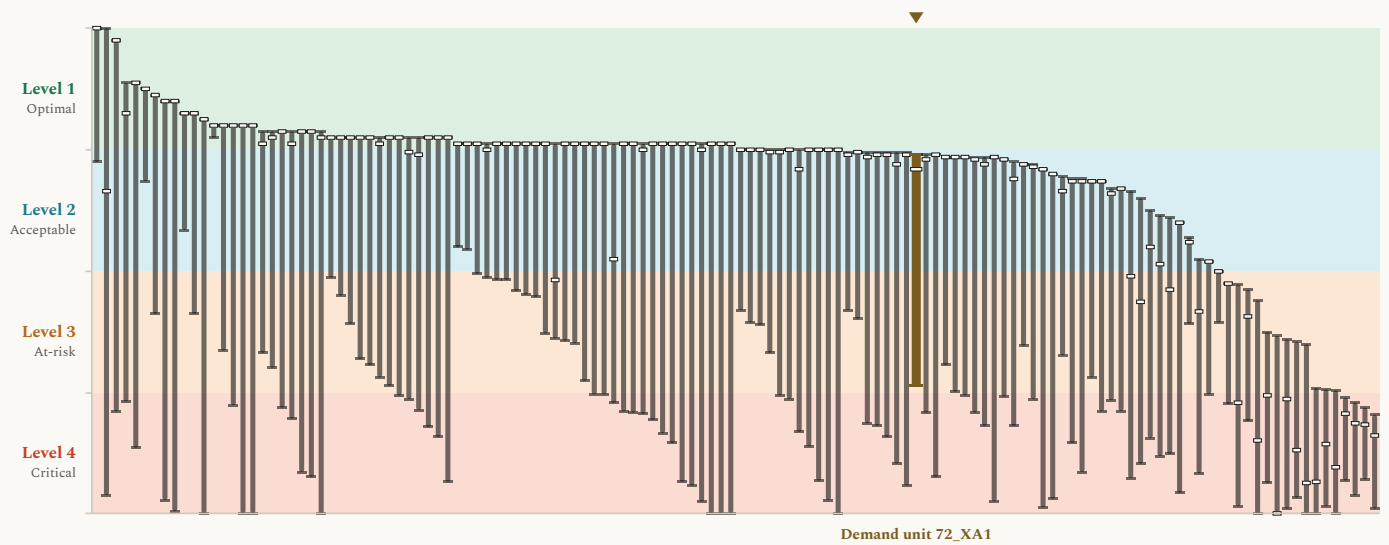
Figure 2. Revenue results, presented as modeled outcome levels, across the 132 agricultural revenue locations, with Demand unit 72_XA1 marked. Each column shows the span of modeled results for one agricultural water service area across the COEQWAL library. Ends of a column are the lowest and the highest modeled value at that location across the runs that report it. A short dash across a column is that location's own baseline (current operations under the historical hydroclimate). This figure uses the same value axis (y-axis) format as Figure 1. Every column uses the same encoding; the column for Demand unit 72_XA1, this brief's subject, is drawn wider, in a distinct color, and marked above. The scale is set out in how to read the values.
