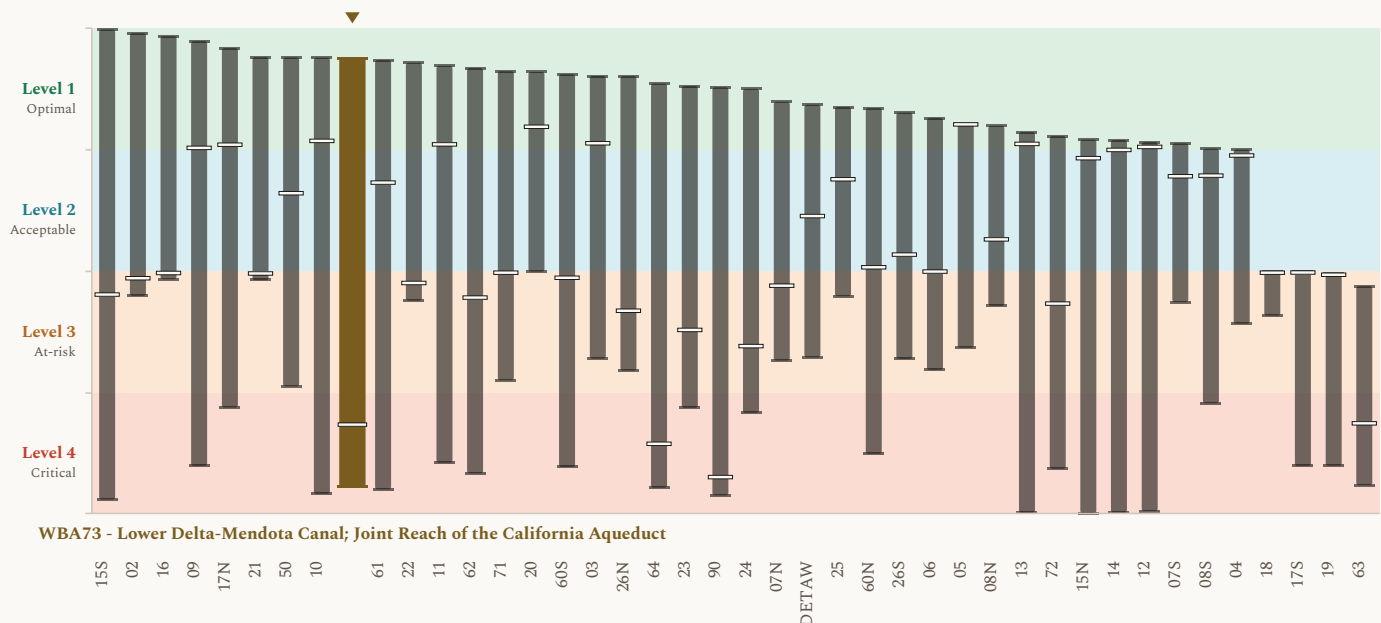
Figure 2. Groundwater storage results, presented as modeled outcome levels, across the 42 groundwater storage locations, with WBA73 - Lower Delta-Mendota Canal; Joint Reach of the California Aqueduct marked. Each column shows the span of modeled results for one groundwater basin area across the COEQWAL library. Ends of a column are the lowest and the highest modeled value at that location across the runs that report it. A short dash across a column is that location’s own baseline (current operations under the historical hydroclimate). This figure uses the same value axis (y-axis) format as Figure 1. Every column uses the same encoding; the column for WBA73 - Lower Delta-Mendota Canal; Joint Reach of the California Aqueduct, this brief’s subject, is drawn wider, in a distinct color, and marked above. The scale is set out in how to read the values.
