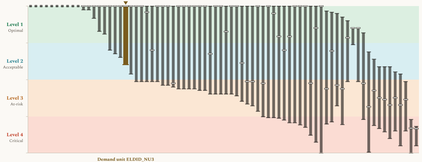
Figure 2. Delivery results, presented as modeled outcome levels, across the 74 community surface water locations, with Demand unit ELDID_NU3 marked. Each column shows the span of modeled results for one community water system across the COEQWAL library. Ends of a column are the lowest and the highest modeled value at that location across the runs that report it. A short dash across a column is that location's own baseline (current operations under the historical hydroclimate). This figure uses the same value axis (y-axis) format as Figure 1. Every column uses the same encoding; the column for Demand unit ELDID_NU3, this brief's subject, is drawn wider, in a distinct color, and marked above. The scale is set out in how to read the values.
